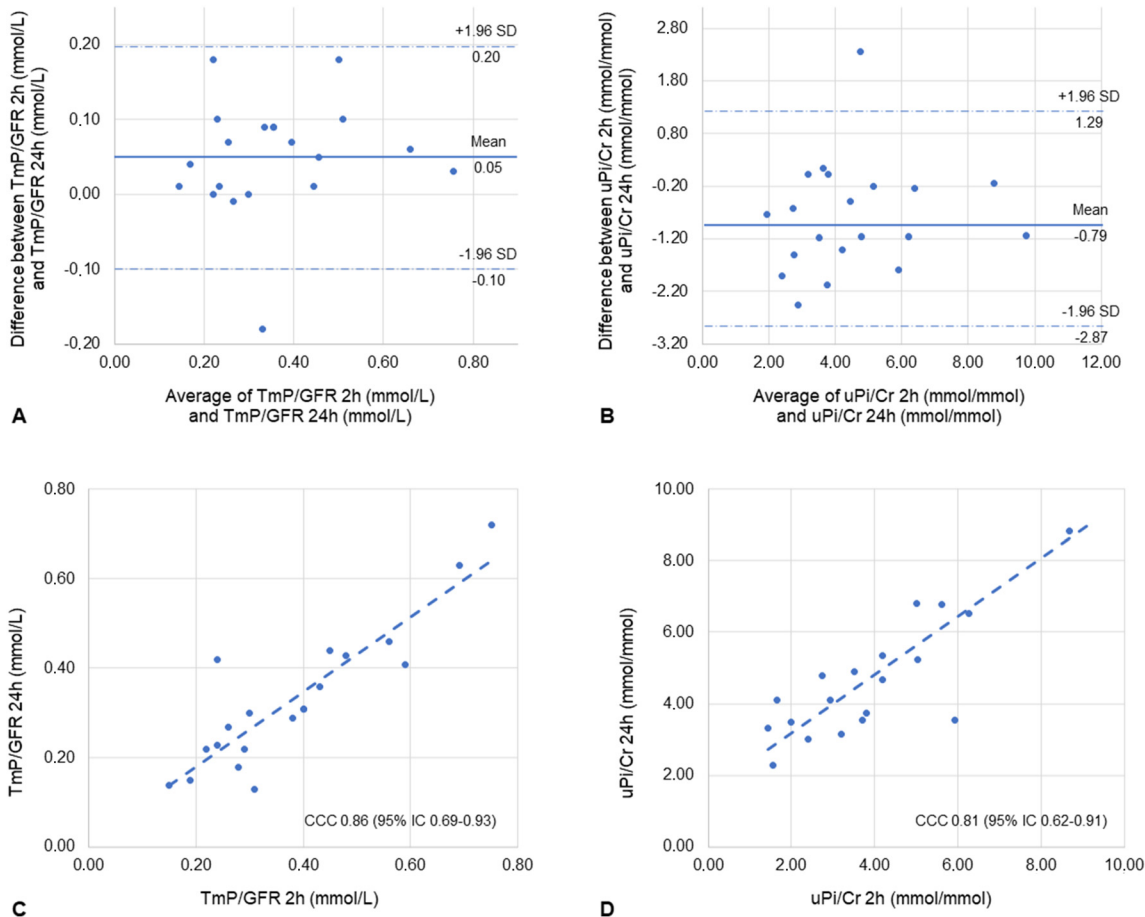
Figure 1: Bland-Altman analysis (A) and Lin's concordance correlation coefficient (C) for TmP/GFR 2 h and TmP/GFR 24 h. Bland-Altman analysis (B) and Lin's concordance correlation coefficient (D) for uPi/Cr 2 h and uPi/Cr 24 h.
