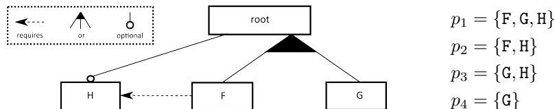
Fig. 1. Feature diagram of running example
