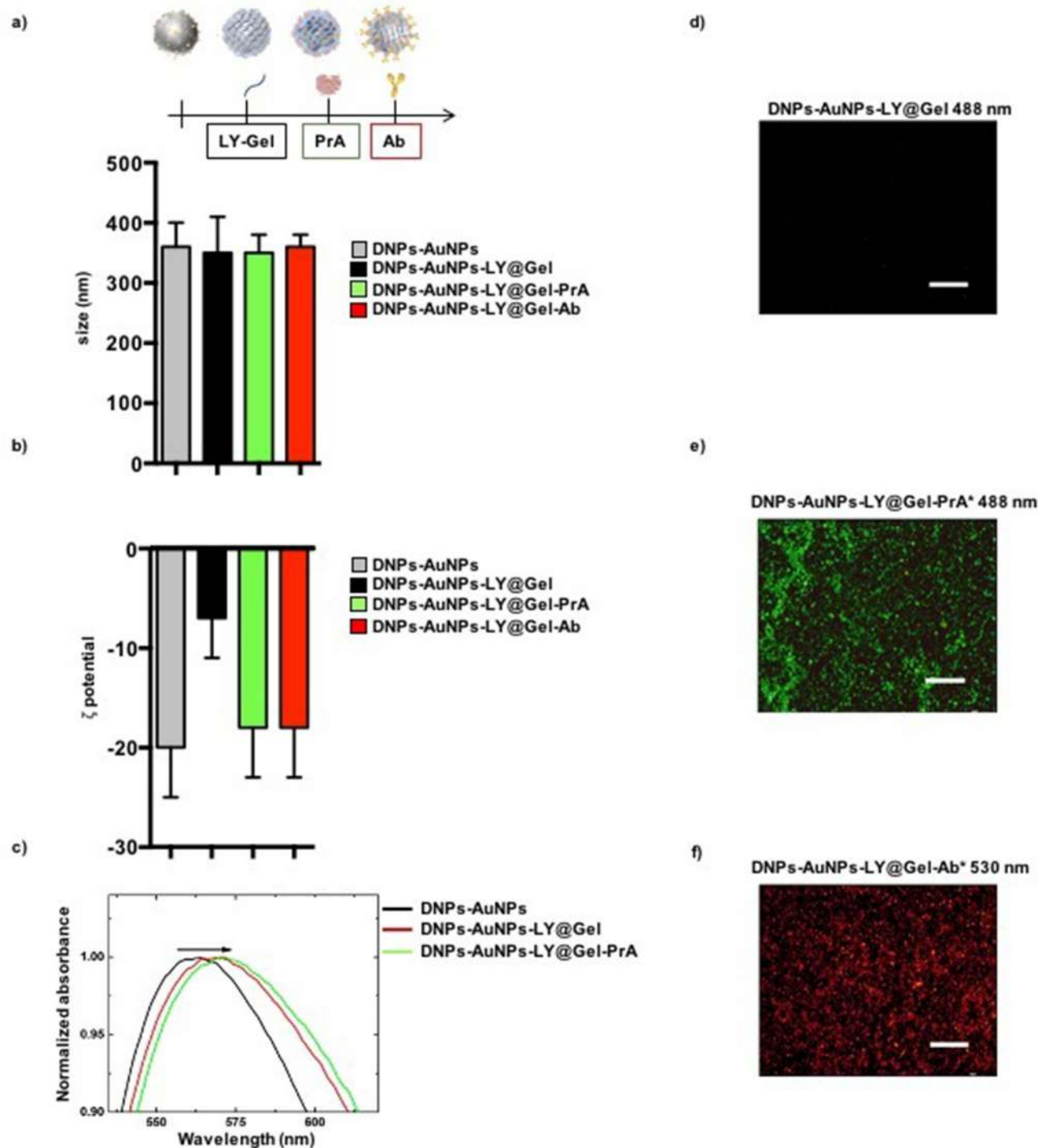
Figure 1 (a) DLS analysis of NPs' size. (b) Analysis of NPs' surface charge. (c) LSPR response of the plasmonic DNPs-AuNPs (black line) after gelatin capping (DNPs-AuNPs-LY@Gel, red line) and further surface modification with the protein A (DNPs-AuNPs-LY@Gel-PrA, green light). (d) Fluorescence microscopy analysis of DNPs-AuNPs-LY@Gel, (e) DNPs-AuNPs-LY@Gel-PrA* both excited at 488 nm, and (f) DNPs-AuNPs-LY@Gel-Ab* excited at 530 nm. The scale bars are 25 μm.
