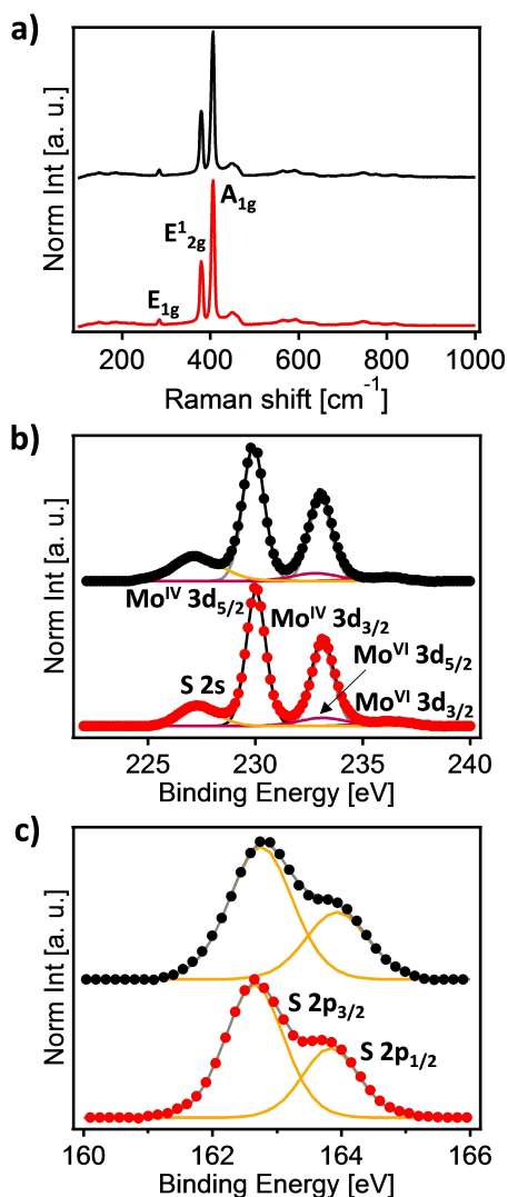
Figure 4. a) Normalized Raman spectra of bulk 2H–MoS 2 (in red) and MoS 2 -50 °C-vac (in black) normalized respect to the A 1g peak of each material (at 532 nm). b) Normalized Mo 3d XPS spectra of bulk 2H–MoS 2 (in red) and MoS 2 -50 °C-vac (in black). c) Normalized S 2p XPS spectra of bulk 2H–MoS 2 (in red) and MoS 2 -50 °C-vac (in black).
