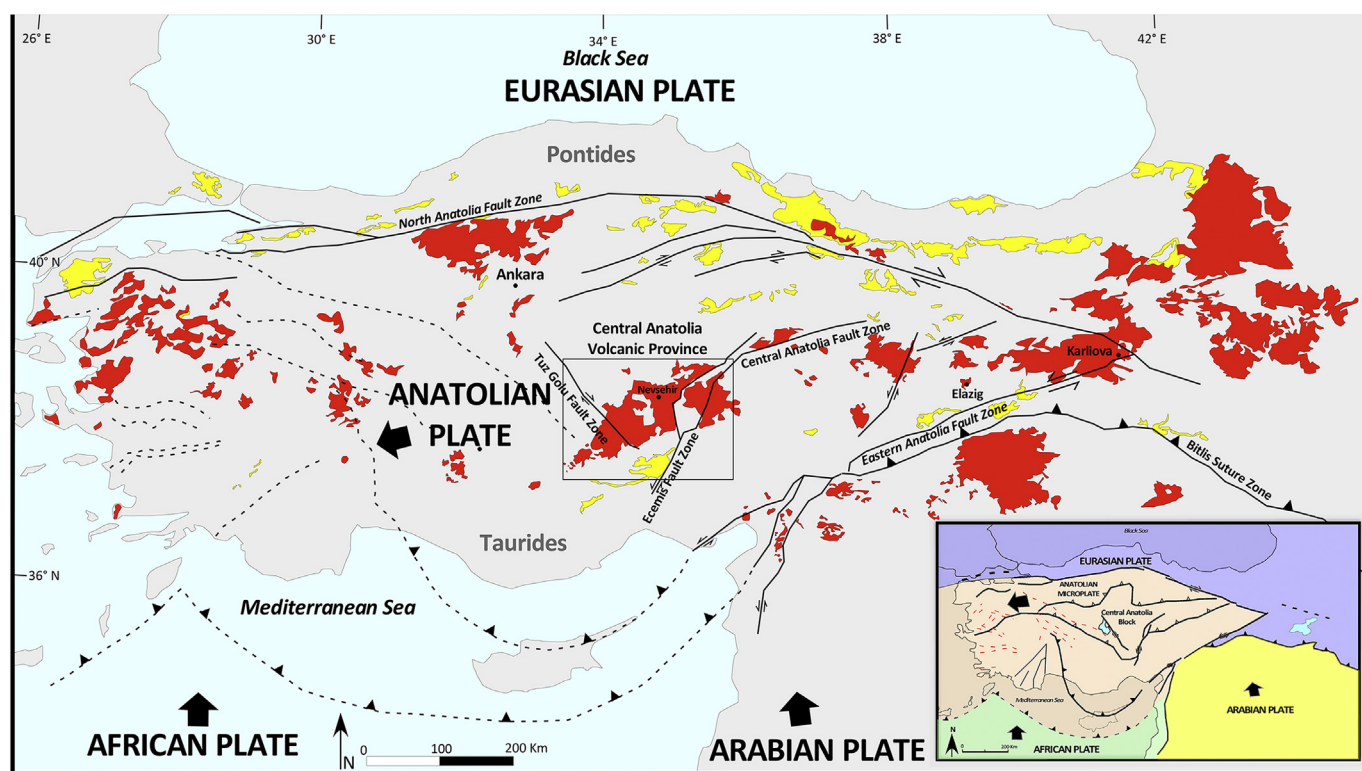
Fig. 1. Sketch map of the Anatolia microplate and adjoining regions showing the main structural features and volcanic activity: Palaeogene volcanism in yellow, Neogene magmatism in red (modified after Uslular et al., 2015). The inset reports the tectonic setting of the region and shows the interaction between the Arabian, African and Eurasian plates. Big arrows represent the motion of the tectonic plates relative to Eurasia. The rectangle delimits the study area (see Fig. 2).
