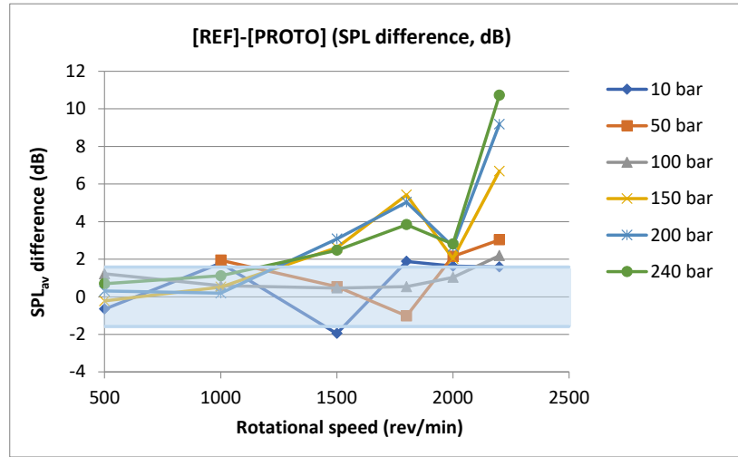
Figure 4.6. SPL_{av} difference between reference and optimized pumps for all the operating conditions
