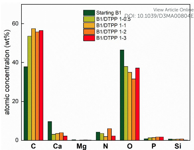
Figure 5. Atomic distributions of elements for the tested specimens
