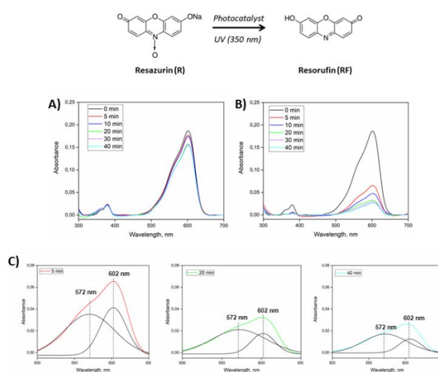
Figure 10. Photocatalytic activity of COTTON-B1(A) and COTTON-B1/DTPP (B) in resazurin aqueous solution under UV irradiation. (C) Deconvoluted spectra after 5, 20 and 40 min of reaction.
