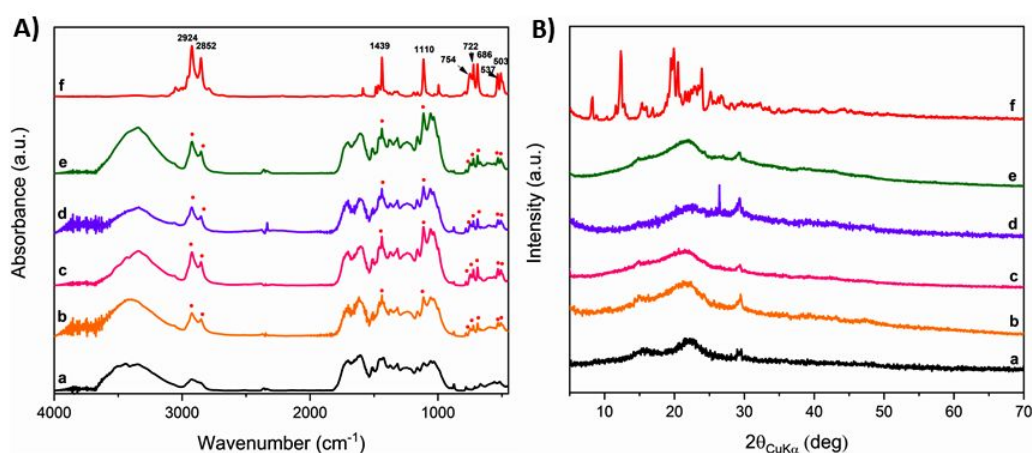
Figure 3. FTIR (A) and WAXD (B) of B1(a), B1/DTPP in a weight ratio of 1/0.5 (b), 1/1 (c), 1/2 (d) 1/3 (e) and DTPPBr (f)
