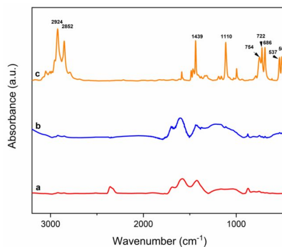
Figure 8. FTIR spectra of (a) B2, (b) B2 after reaction with DTPP, and (c) DTPPBr
