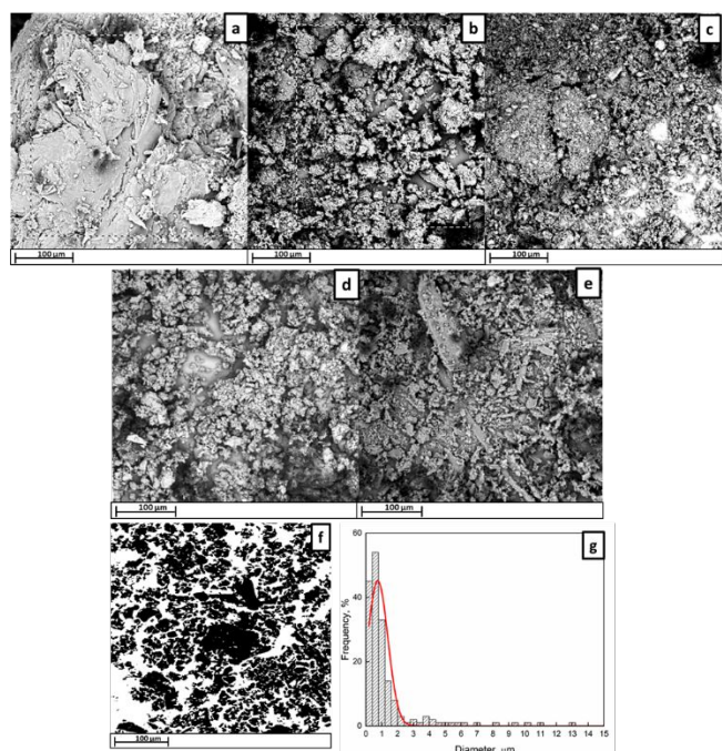
Figure 4. SEM/EDX images of different B1/DTTP samples: A) starting B1, B) B1/DTTP prepared in ratio 1 to 0.5, C) B1/DTTP prepared in ratio 1 to 1, D) B1/DTTP prepared in ratio 1 to 2, E) B1/DTTP prepared in ratio 1 to 3, F) sample image analysis of B1/DTTP 1 to 2 and G) mean size distribution of B1/DTTP 1 to 2.
