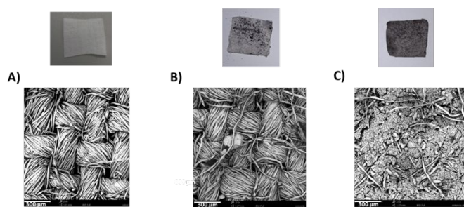
Figure 9. Pictures and SEM images of A) cotton fabric, B) COTTON-B1, and C) COTTON-B1/DTPP
