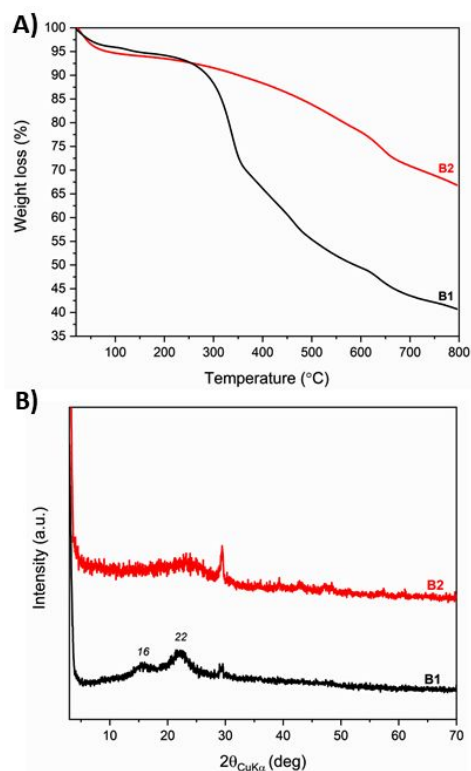
Figure 2. TGA (A) and X-ray diffraction pattern (B) of B1 and B2
