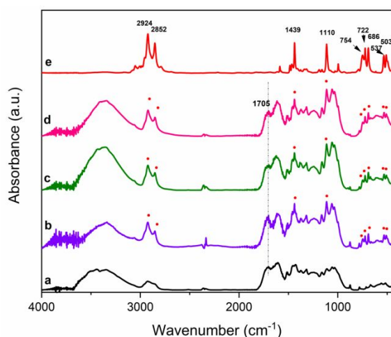
Figure 7. FTIR spectra of: (a) B1, (b) B1/DTPP milled with Silicon nitride, (c) tempered steel, (d) zirconia balls, and (e) DTPPBr
