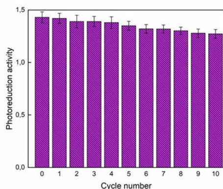
Figure 11. Reusability tests of COTTON-B1/DTPP.
