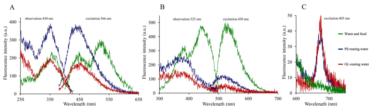
Fig. 4. Spectrofluorimetric analysis of rearing water before and after larval development. Excitation and emission spectra recorded from rearing water containing larval food before (green; control condition) and after larval development in PS (blue) and GL (red) containers. Spectra were acquired under different combinations of excitation and emission conditions (A and B) or under excitation at 405 nm (C), as indicated in the respective panels.
