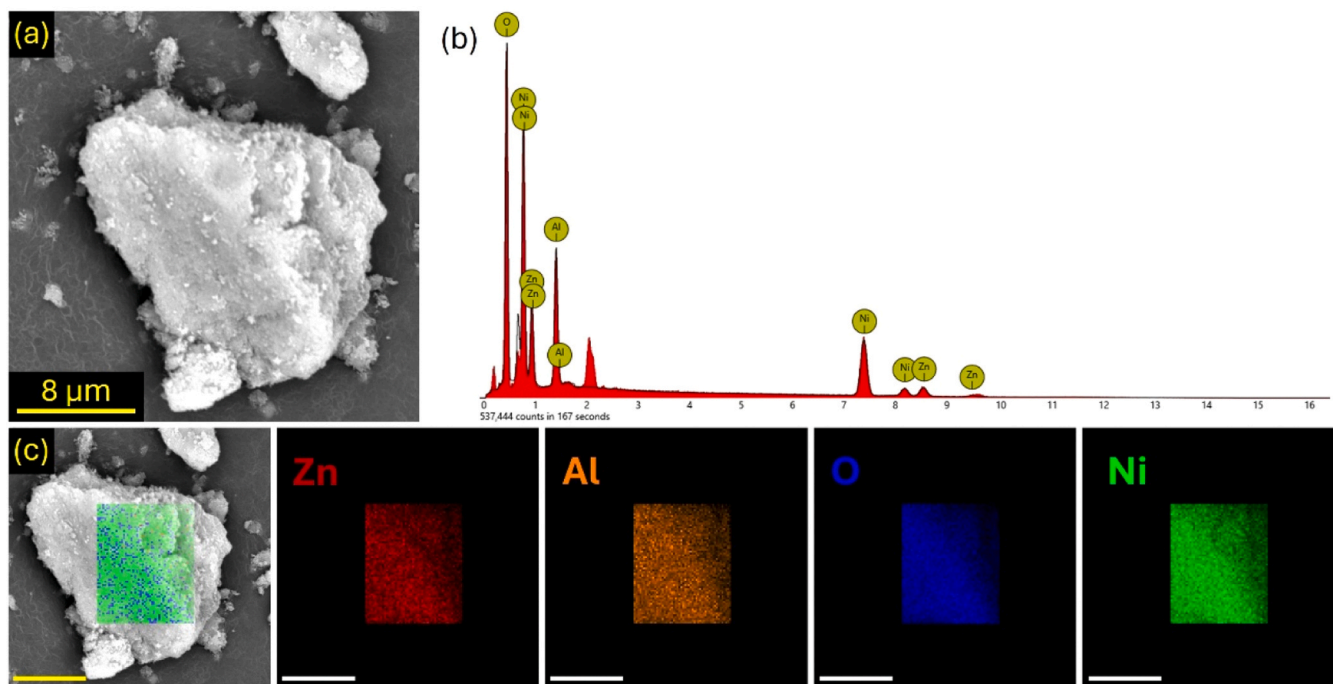
Fig. 6. SEM image (a), EDX spectrum (b) and elemental mapping (c) of Ni-Zn-Al LDHd sample (scale bar 8 \mu m).
