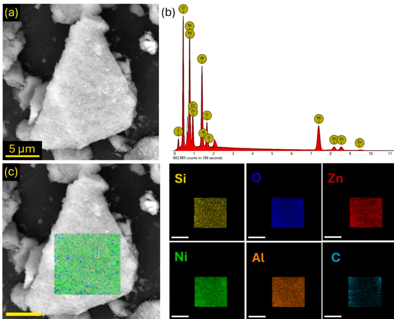
Fig. 7. SEM image (a), EDX spectrum (b) and elemental mapping (c) of Ni-Zn-Al LDHd + HAL200 (2:1) sample (scale bar 5 \mu m).
