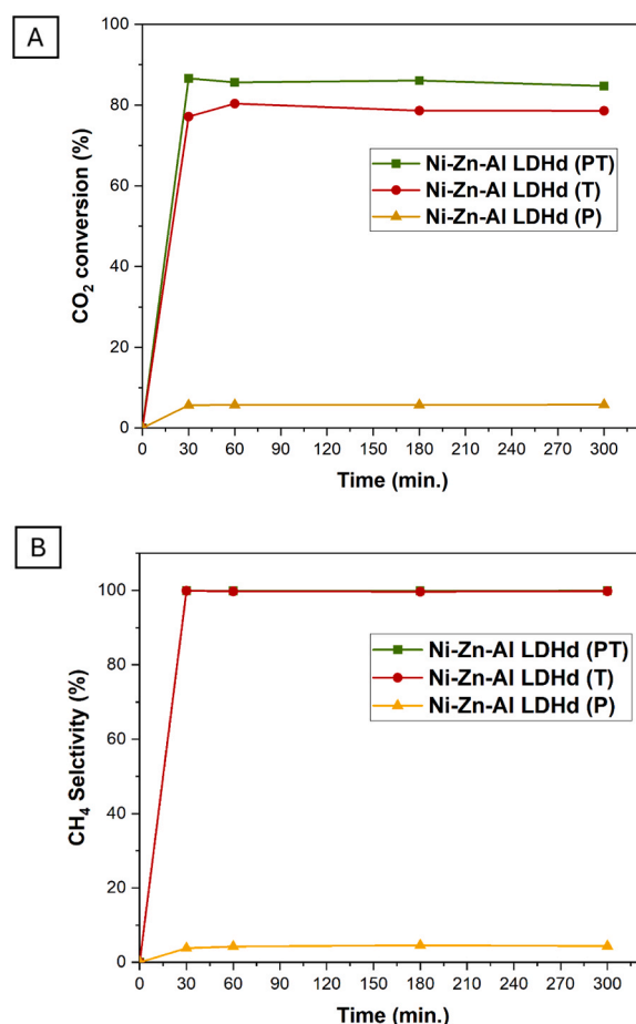
Fig. 1. CO 2 conversion (A) and CH 4 selectivity (B) for Ni-Zn-Al LDHd catalyst tested in Photothermo-catalytic (PT), Thermocatalytic (T) and Photocatalytic (P) CO 2 methanation reaction at atmospheric pressure. The reaction temperature was 350 °C for the PT and T processes, whereas for the P process the temperature was 200 °C (reached only with the use of the solar lamp).
