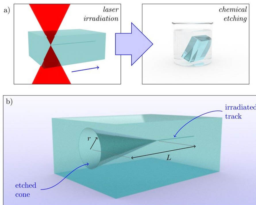
Figure 1. (a) Pictorial representation of the two steps of the laser-assisted etching process. First (left panel), tracks are irradiated with a focused femtosecond laser beam, in the bulk of a glass sample and covering its full length. The irradiation is performed by translating the sample at constant speed with respect to the laser focus. Second (right panel), the sample is immersed in a solution of HF or KOH for a controlled time. (b) Typical outcome of the etching process of a straight irradiated track. A hollow cone is formed along the track, with basis radius r and length L . The aspect ratio (A.R.) of the cone, defined as A.R. = L/r , is a direct indication of the etching selectivity. Dimensions are not to scale.
