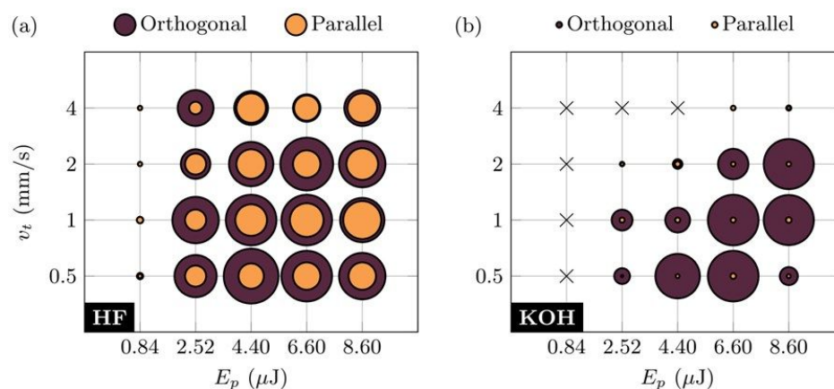
Figure 2. Characterisation of the A.R. of the etched cones as a function of the irradiation parameters: pulse energy E_p , translation speed v_t , and polarisation (parallel or orthogonal with respect to the translation direction). The repetition rate of the laser pulses is 25 kHz. The area of the coloured circles indicates the A.R. of the cones, as measured (a) after 10 min of etching in HF solution or (b) after 6 h in KOH solution. The size of the circles in the legend corresponds to a value of 10.
