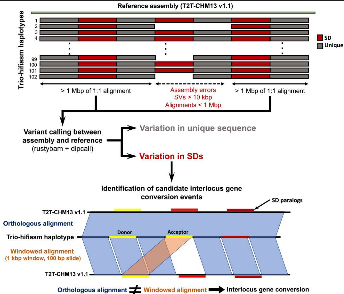
Extended Data Fig. 1 | Analysis schema for variant and IGC calling. Whole-genome alignments were calculated for the HPRC assemblies against T2T-CHM13 v1.1 with a copy of GRCh38 chrY using minimap2 v2.24. The alignments were further processed to remove alignments that were redundant in query sequence or that had structural variants over 10 kbp in length. After these steps, the remaining alignments over 1 Mbp were defined to be syntenic and used in downstream analyses. We then counted all pairwise single-nucleotide differences between the haplotypes and the reference and stratified these results into unique regions versus SD regions based on the SD annotations from T2T-CHM13 v1.1. All variants intersecting tandem repeats were filtered to avoid spurious SNV calls. To detect candidate regions of IGC, the query sequence with syntenic alignments was fragmented into 1 kbp
