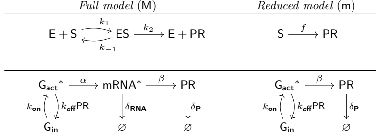
Fig. 3. Example models tested in this paper. Top panel: the Henri-Michaelis-Menten model, where \mathbf{m} is derived when \mathbf{C} : [E]_0 + [ES]_0 \ll [S]_0 + K_{\text{MM}} . Bottom panel, a protein translation network where \mathbf{m} when \mathbf{C} : \beta \gg \alpha .
