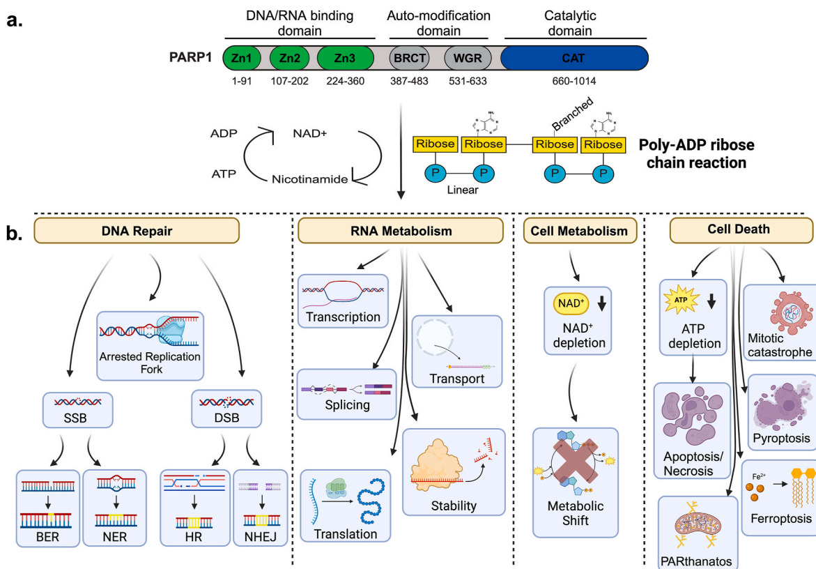
Fig. 1. Schematic representation of PARP1 structure and its intracellular functions.
