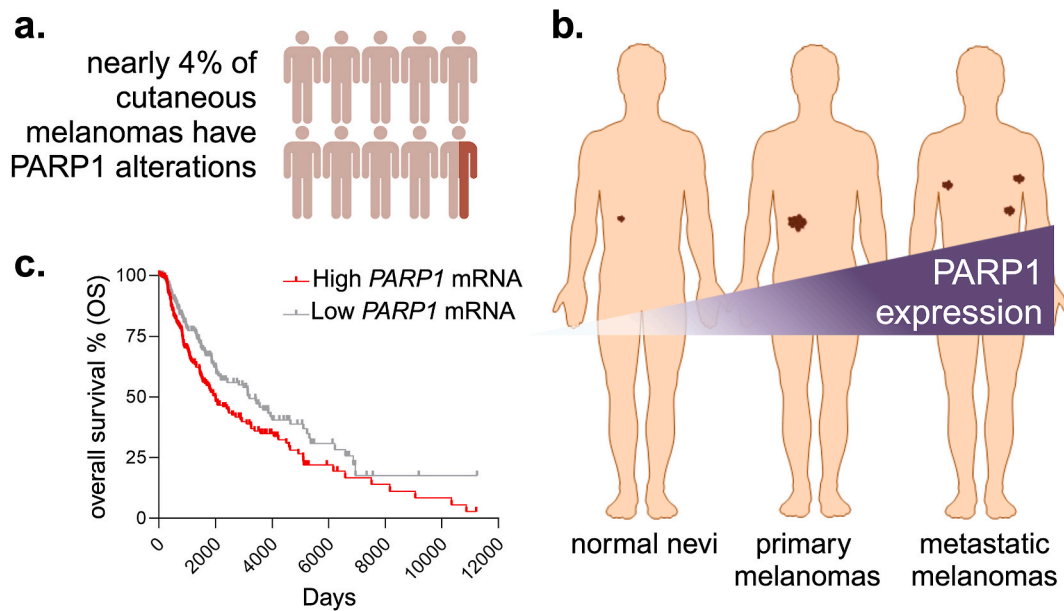
Fig. 2. PARP1 in melanoma.
