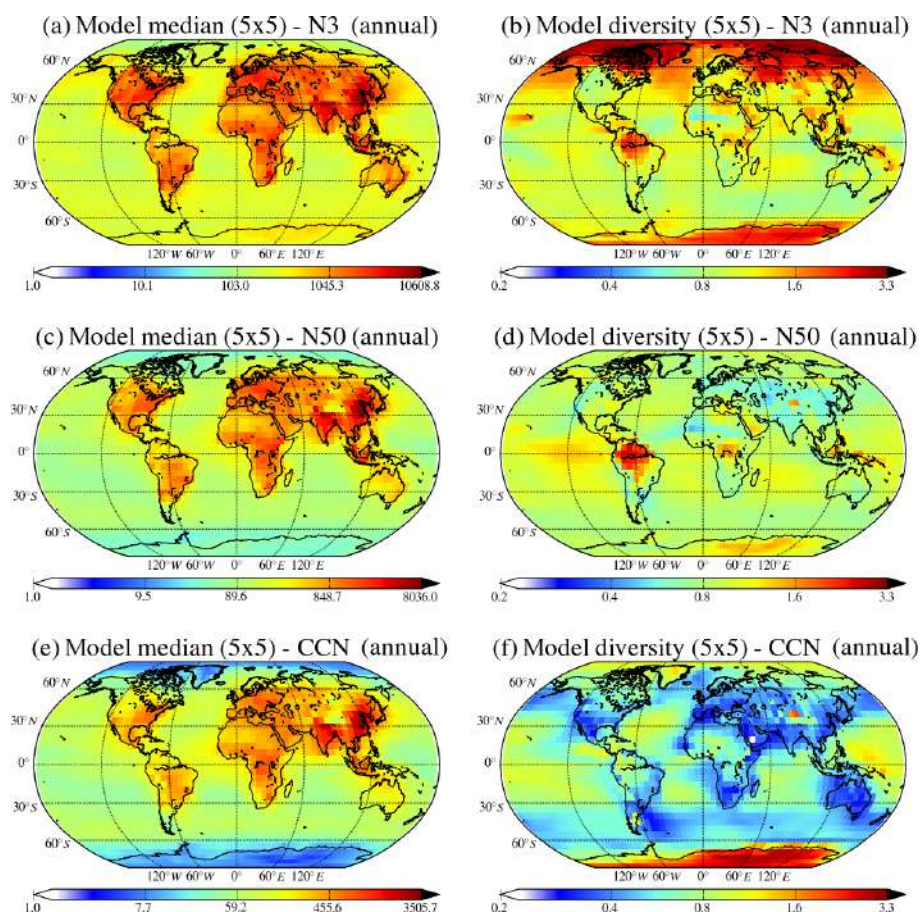
Figure 10. Global distributions of the annual multi-model median concentrations of N_3 , N_{50} and CCN_{0.2} ( \text{cm}^{-3} ) for the year 2011 (a, c, e, respectively) and the corresponding diversities (b, d, f, respectively; calculated as the ratio of standard deviation to the mean of the models).
