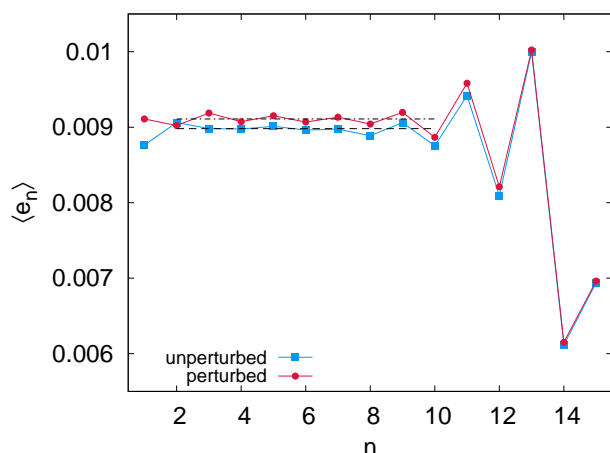
FIG. 10. Energy spectra of unperturbed and perturbed inviscid Sabra shell model. The fit to the equiparted region of the spectra, pertaining to the shells which are far enough from the lower boundary, lead to the value R_{corr}^{(\infty)} . Initial perturbation \delta_{m=7} \simeq 1.79 \cdot 10^{-3} .
