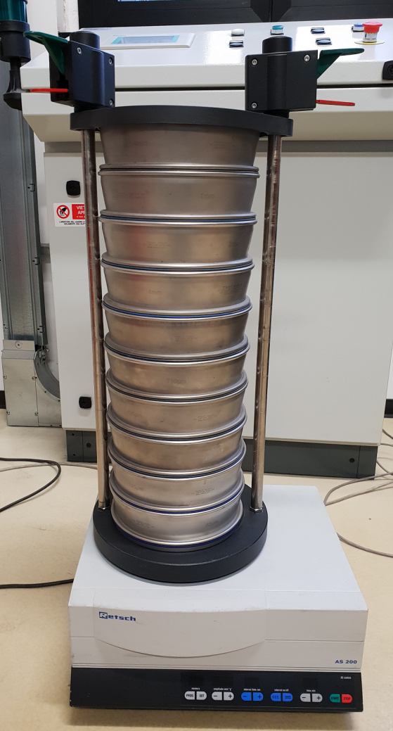
Figure 3: Analytic sieve AS200.
