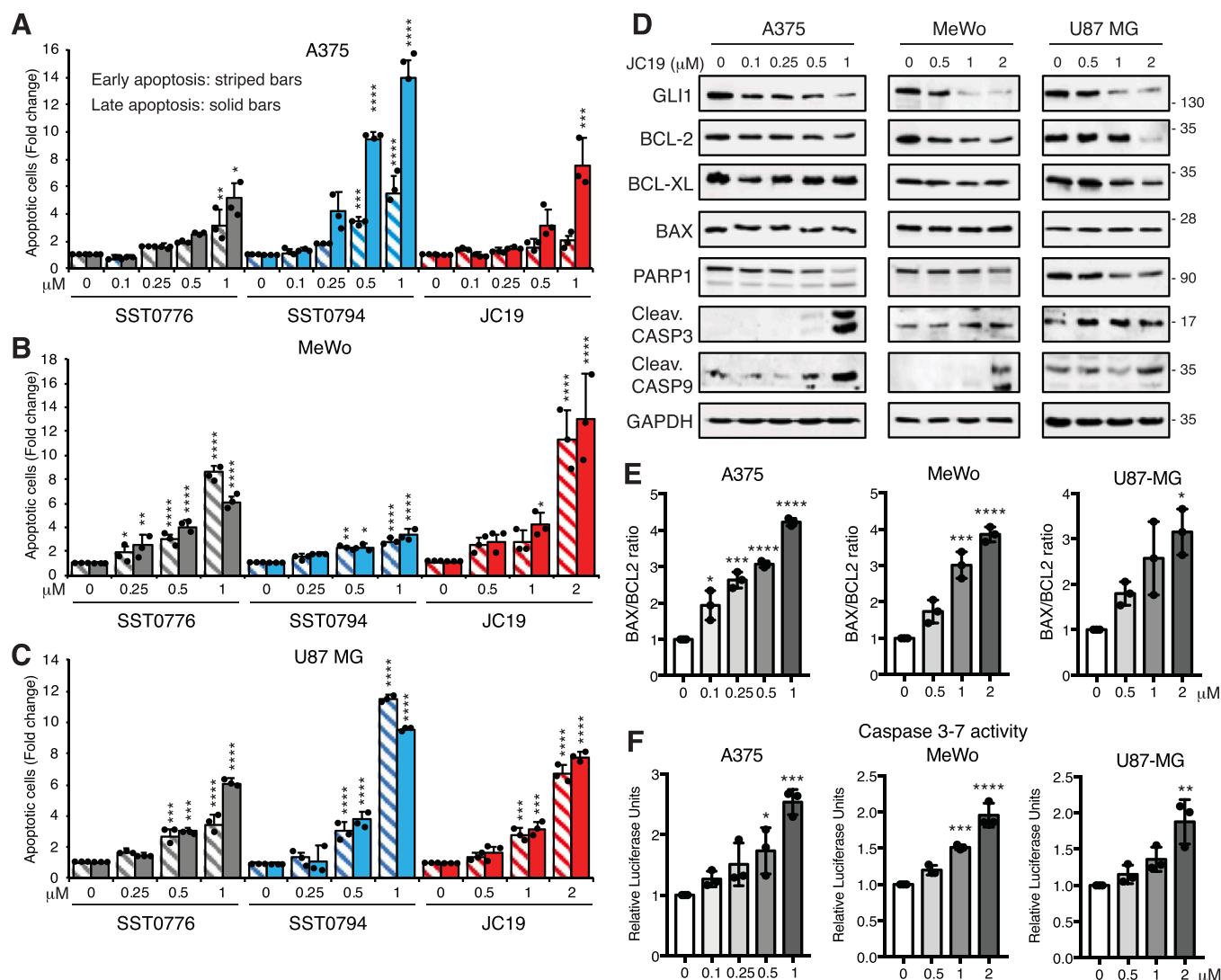
Fig. 4. GLI inhibition induces apoptosis in cancer cells. A-C) AnnexinV/7-AAD double staining of early (AnnexinV+/7-AAD-) and late (AnnexinV+/7-AAD+) apoptosis of A375 (A), MeWo (B), and U87-MG (C) cells treated with increasing doses of SST0776, SST0794, and JC19 for 72 h, with cells treated with DMSO equated to 1. D) Western blot of GLI1, BCL-2, BCL-XL, BAX, PARP1, cleaved Caspases 3 and 9 in A375, MeWo, and U87-MG cells treated with increasing doses of JC19 for 72 h. GAPDH was used as loading control. E) Densitometric quantification of BAX/BCL2 ratio as shown in D. F) Activity of Caspase 3 and 7 in A375, MeWo and U87 cell lines treated with increasing doses of JC19 for 72 h. Cells treated with DMSO were equated to 1. *, p < 0.05 ; **, p < 0.01 ; ***, p < 0.001 ; ****, p < 0.0001 (one-way ANOVA). Data represent mean \pm SD of at least three independent experiments.
