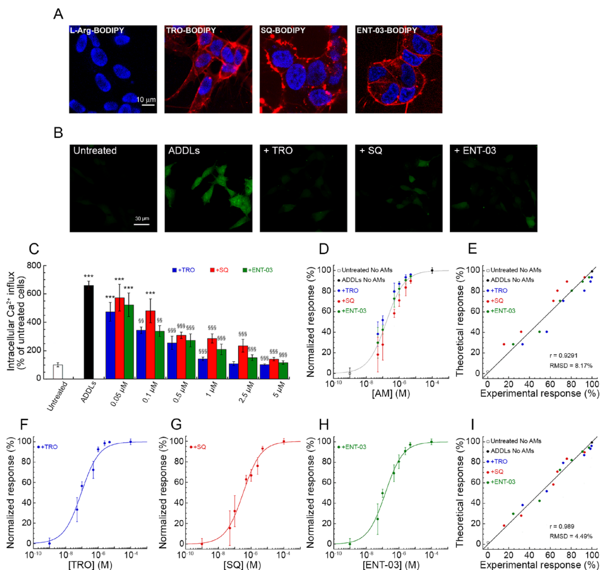
Figure 9. The three AMs bind to the plasma membrane of SH-SY5Y cells and prevent the increase of intracellular \text{Ca}^{2+} levels induced by ADDLs (global fitting analysis). (A) Representative confocal microscopy images (median planes parallel to the coverslip) of SH-SY5Y cells incubated for 30 min at room temperature with 5 \mu\text{M} of L-Arg-BODIPY, TRO-BODIPY, SQ-BODIPY, or ENT-03-BODIPY (probe:molecule of 1:10). Blue and red fluorescences indicate Hoechst-labeled nuclei and AM-BODIPY, respectively. (B) Representative confocal scanning microscopy images of free \text{Ca}^{2+} levels in untreated SH-SY5Y cells or in cells treated for 15 min with 1 \mu\text{M} ADDLs in the absence or presence of 1 \mu\text{M} AMs. (C) Intracellular free \text{Ca}^{2+} -derived fluorescence in untreated SH-SY5Y cells or in cells treated for 15 min with ADDLs in the absence or presence of the indicated concentrations of AMs. Experimental errors are SEM ( n = 4 ). *** symbols refer to p values < 0.001 relative to untreated cells. §§ and §§§ symbols refer to p values < 0.01 and < 0.001 , respectively, relative to ADDLs without AMs. (D) Normalized dose–response curve obtained from \text{Ca}^{2+} -derived fluorescence data of all AMs in panel C and fitted to eq 2. (E) Plot reporting theoretical versus experimental response values obtained from eq 2. (F–H) Normalized dose–response curves for TRO (blue), SQ (red), and ENT-03 (green) obtained from \text{Ca}^{2+} -derived fluorescence data in panel C. In each plot, the lines through the data do not represent independent fitting procedures using eq 2, but result from global fitting using only eq 4, in all cases with corresponding values of \zeta potential, BTF, and FRET data. Experimental errors are SEM ( n = 4 ). (I) Plot reporting theoretical versus experimental response values obtained from eq 4.
