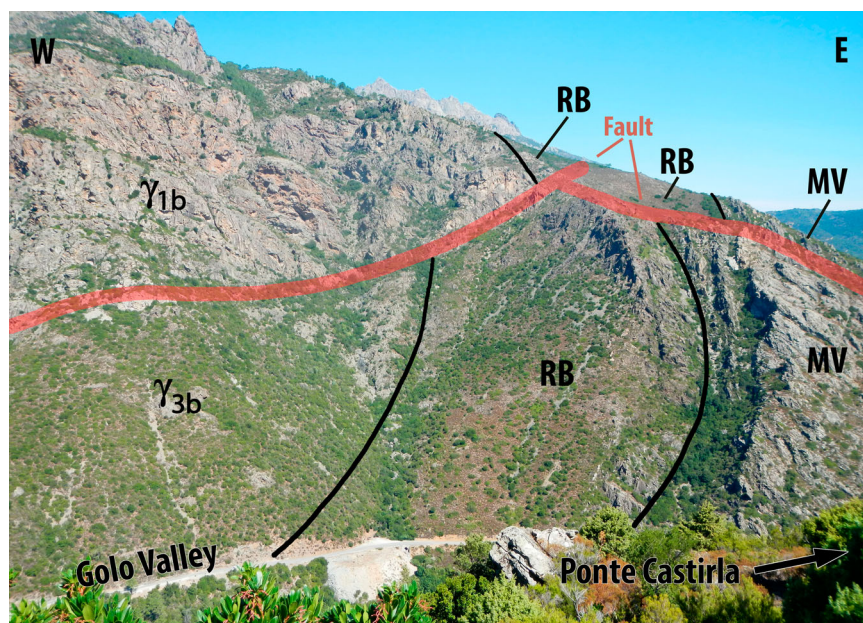
Figure 4. View of the contact between the HC and AC along the Golo Valley. The contact is represented by a deformed, steep surface that upward becomes overturned. Legend: \gamma_{1b} : Pink granites (U3 suite); \gamma_{3b} : monzogranites (U2 suite); RB: Roches Brune Fm.; MV: Metavolcanites and Metavolcaniclastites Fm.
