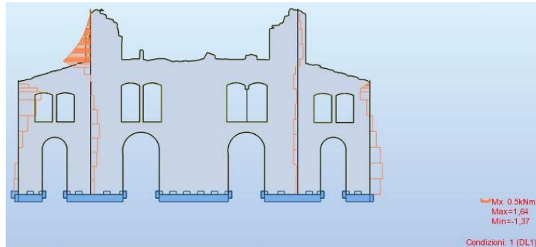
Fig. 9. A structural analysis result of a Fornace Penna facade from the BIM model.
