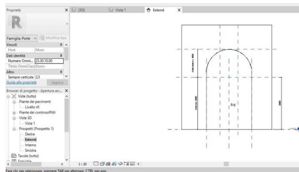
Fig. 3. An example of a parametrization of an arc opening in BIM.
