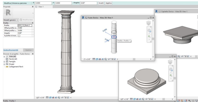
Fig. 7. Nested Family “Column” containing three families: capital, shaft and base. Each family includes profile families.
