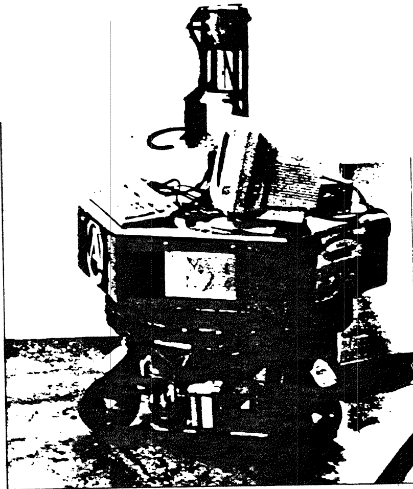
Figure 1: CARMEL stands just under a meter tall and moves at speeds up to 780 mm/sec. A ring of 24 sonars surround the robot's torso; a grayscale CCD camera mounted on a rotating tower provides visual capabilities. The monitor and keyboard are used for debugging, and not used in actual competition.
