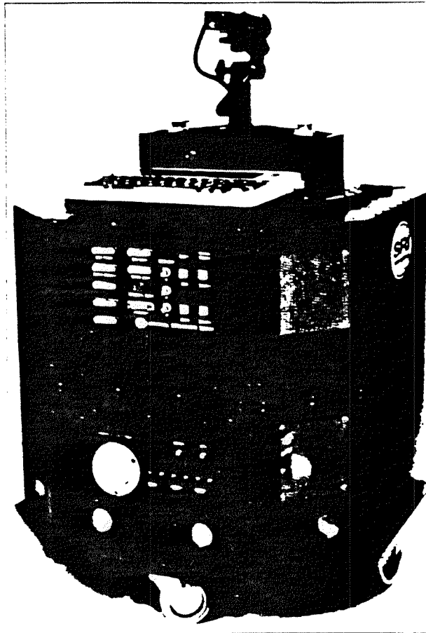
Figure 2: Flakey is about one meter high and moves at speeds up to 500 mm/sec. Twelve sonars (four in front, four in back, and 2 at each side), and eight touch-sensitive bumpers surround the robot. A structured-light sensor provides a dense depth map over a small region in front of Flakey.
