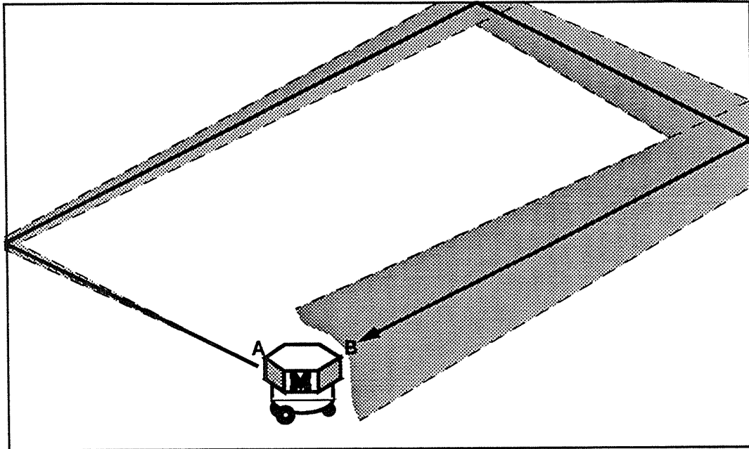
Figure 5: Crosstalk occurs when a sonar sensor picks up stray echoes from other onboard sonars. For example, when sonar A is fired, the sounds may reflect against walls; the reflected sound may be picked up by sonar B. Sonar B is unable to distinguish this from its own reflected signal.
