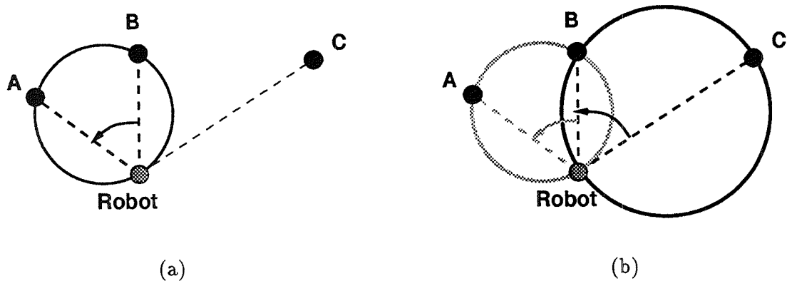
Figure 15: Three-object triangulation can be used to recalibrate the robot's position when dead-reckoning errors have accumulated. To use this method, the locations of three objects A, B, and C are known, and the directions to the three objects from the perspective of the robot are known; the robot's location is unknown. In (a), objects A and B, plus the angle between them (relative to the robot) are used to calculate a circle; the robot is somewhere on the perimeter of this circle, but its exact location is not yet known. In (b), a second circle is similarly calculated, using objects B and C. The two circles intersect at two points: the location of object B and the location of the robot.
