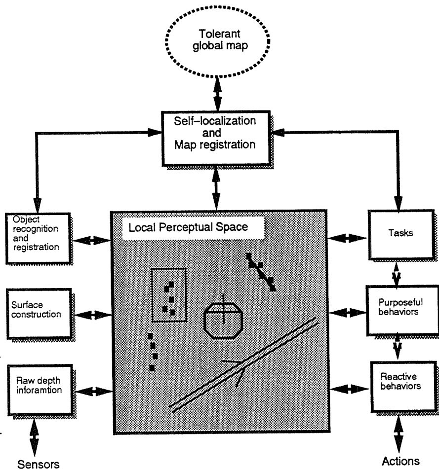
Figure 4: Flakey's system architecture has multiple routines updating and referring to the local perceptual space; these routines operate in parallel. In this illustration, perceptual routines are on the left, and action routines are on the right. The vertical dimension gives an indication of the cognitive level of processing, with high-level behaviors and perceptual routines at the top. A map-location module continuously matches local perceptual information to a stored global map, updating Flakey's global position. All modules operate independently in a distributed fashion.
