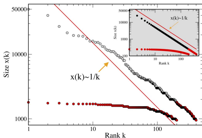
Figure 2 | Zipf's Law for the Richest Billionaires in the United States. The richest 390 persons in the US are billionaires whose wealth we plot against their rank as the uppermost set of points (the first 195 richest being grey circles, the second 195 poorest being red circles). The second set is the sub-sample that we translate to the original ranks and plot as the set of red circle points below the diagonal straight line which is the pure Zipf plot associated with x(k) = x_M/k . The inset is a pure Zipf plot dimensioned to the entire set of 390 billionaires and the poorest sub-sample of 195. (Source: Forbes List http://www.forbes.com/ ).
