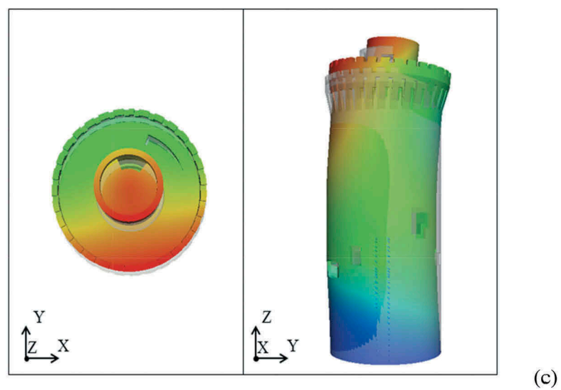
Figure 15. Finite element model: (a) first mode shape; (b) second mode shape and (c) fourth mode shape. The y axis is approximately in the N-S direction and the x axis is in the E-W direction.
