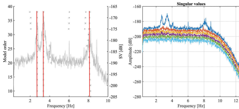
Figure 23. Stabilization diagram of the SSI-cov automated procedure and FDD (acquisition of the 12th of March at 14:15).
