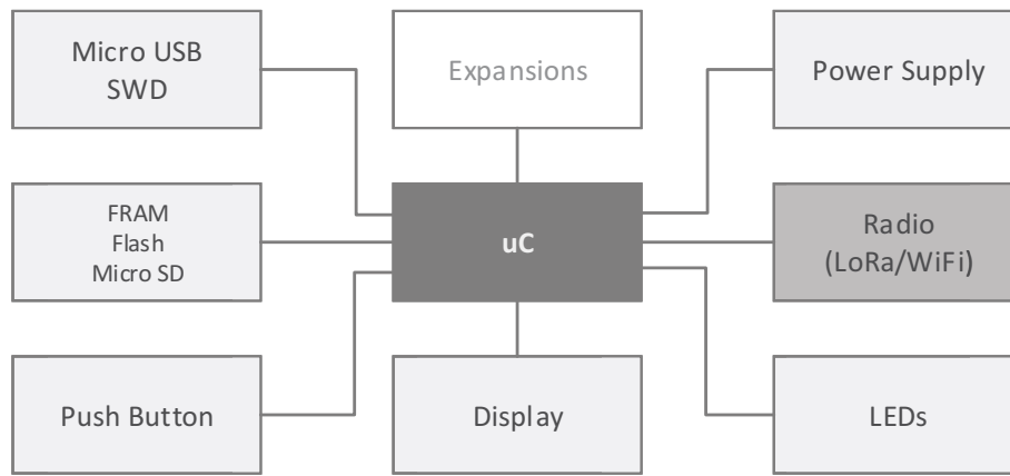
Figure 5. Block diagram of the core module.
