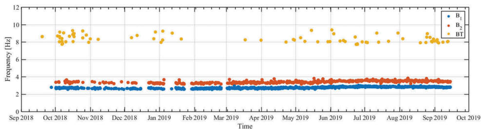
Figure 25. Modal tracking of the identified frequency for each mode.
