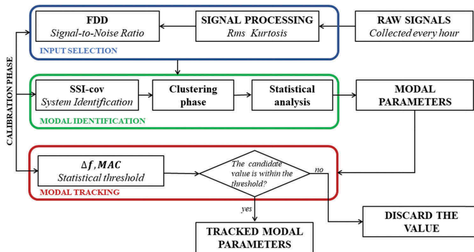
Figure 17. Flowchart of the automated modal identification algorithm.
