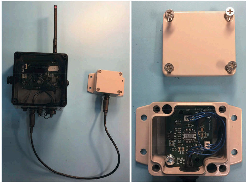
Figure 7. The accelerometer node with custom sensor board and box.
