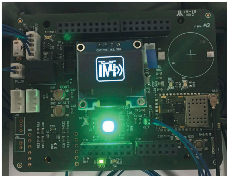
Figure 6. Node display, LEDs and push buttons.
