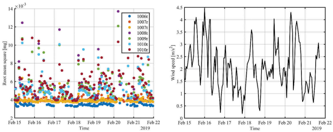
Figure 19. Root mean square values and wind speed over the second calibration period (#P2 3/12/2018-10/12/2018).
