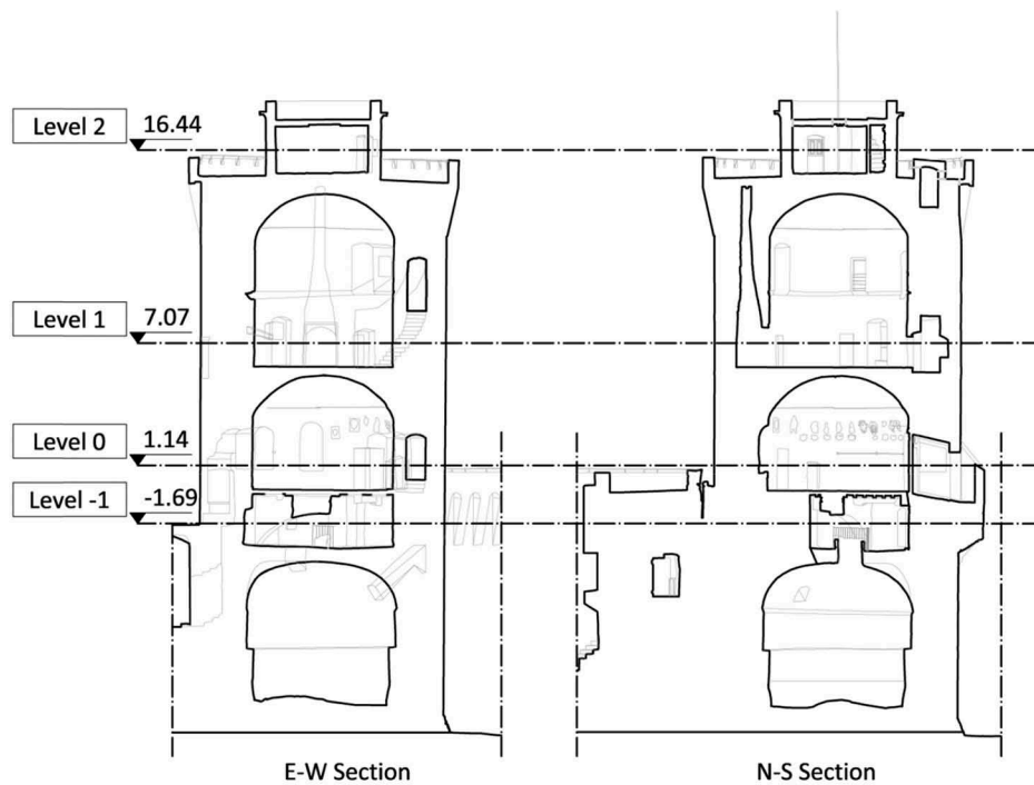
Figure 11. Longitudinal and transversal section of the Matilde Tower.
