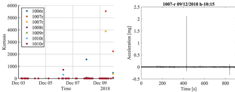
Figure 21. High values of the Kurtosis usually imply spikes or dropouts in the signals.
