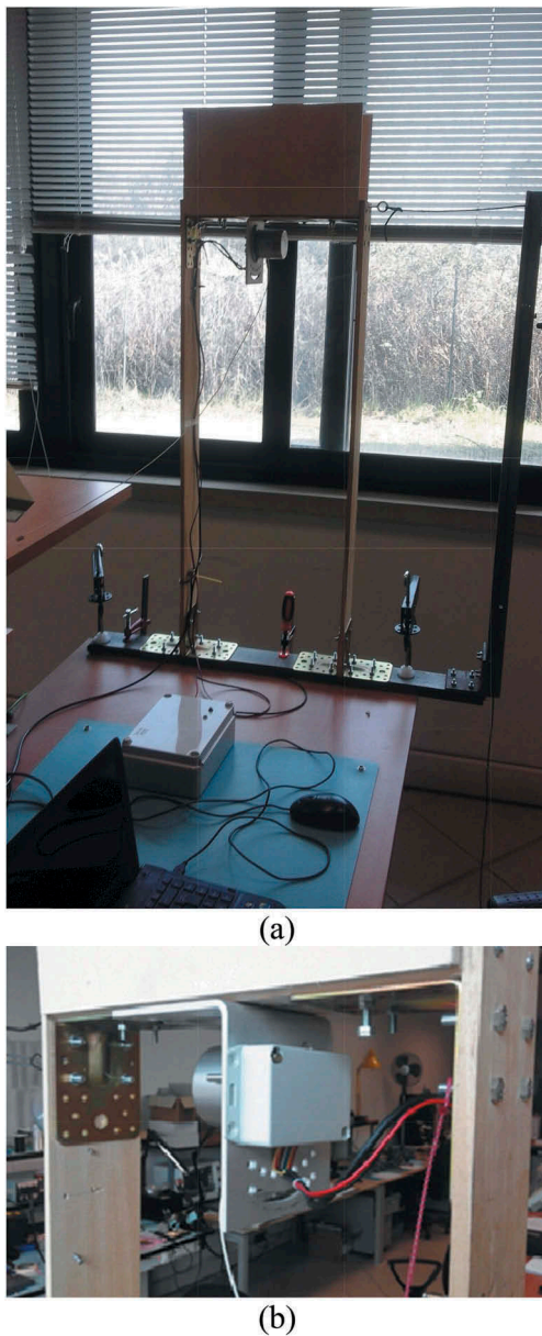
Figure 8. The wooden oscillating structure used for the validation (a) and the developed accelerometer (b).
