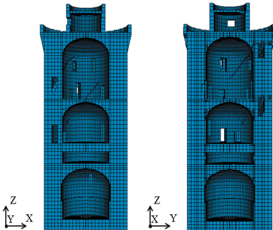
Figure 14. Finite-element model of the Matilde Tower. The y axis is approximately in the N-S direction and the x axis is in the E-W direction.
