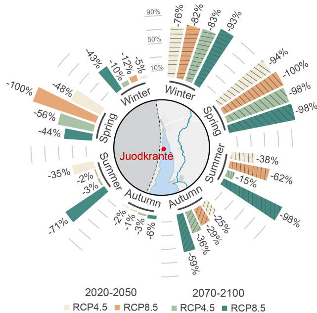
Figure 8. The percentage of change in the seasonal average salinity of saltwater intrusions (solid pattern; left) and number of days on which the salinity exceeded the 2 \text{ g kg}^{-1} threshold (hatched pattern; right) in Juodkrantė, which is approximately 20 km below the strait connecting the Baltic Sea and the Curonian Lagoon. Values denote the percentage of difference in the scenario runs compared with the historical period (1975–2005).
