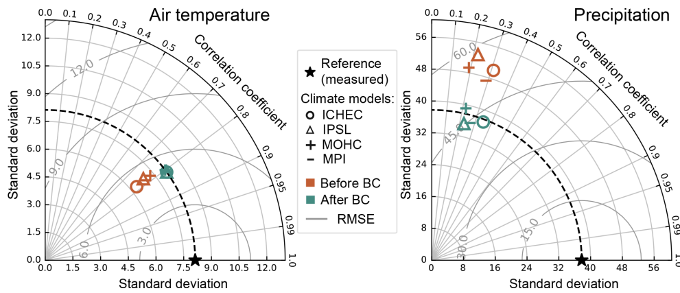
Figure 4. Taylor diagram showing a statistical comparison of air temperature (daily mean) and precipitation (monthly sum) before and after the bias correction (BC) with respect to the reference measurement data. Statistics were computed for the period of 1990–2005.
