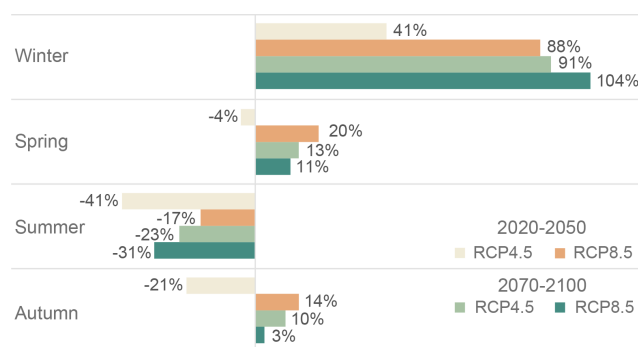
Figure 5. The percentage of change in the seasonal average discharge from the Nemunas river for the RCP4.5 and RCP8.5 scenario runs during the short-term (2020–2050) and long-term periods (2070–2100), compared with the historical period (1975–2005).
