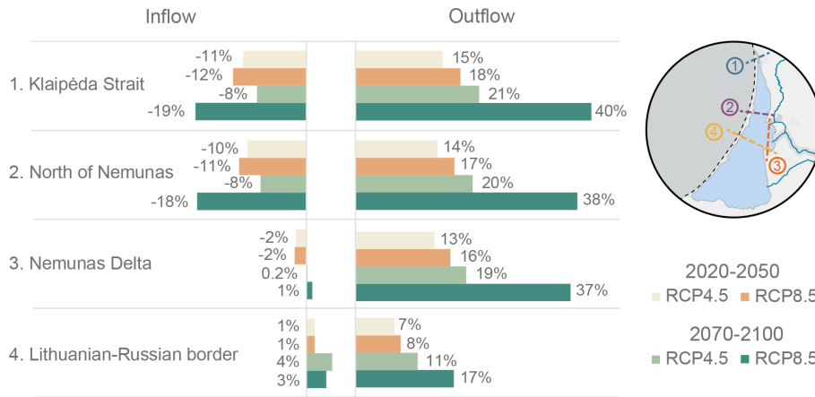
Figure 7. The percentage of change in the projected (under the RCP4.5 and RCP8.5 scenarios) inflowing and outflowing water flux from the historical period (1975–2005). The map insert shows the locations of the predefined cross sections, which include the following 1 – Klaipėda Strait; 2 – north of Nemunas; 3 – Nemunas delta; 4 – Lithuanian–Russian border. Outflow is from south to north (sections 1, 2, and 4) and from east to west (section 3), and vice versa for inflow.
