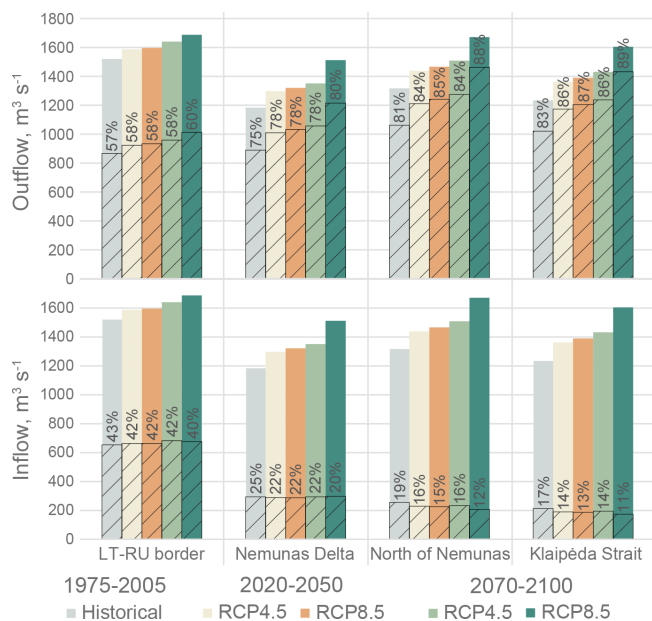
Figure 6. Average outflowing and inflowing water volume (hatched pattern), including its percentage of the absolute flux (solid pattern) of each analysis period, namely historical (1975–2005), short term (2020–2050), and long term (2070–2100), under the RCP4.5 and RCP8.5 scenarios. The locations of the cross sections are shown in Fig. 7.
