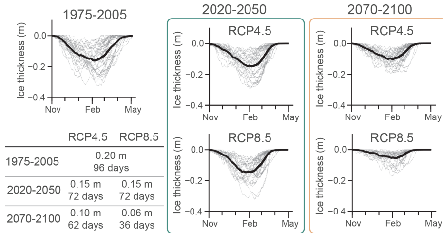
Figure 9. The average ice thickness in the Curonian Lagoon. The black line indicates the average ice thickness of each analysis period, namely historical (1975–2005), short term (2020–2050), and long term (2070–2100) under the RCP4.5 and RCP8.5 scenarios. The table shows the average maximum ice thickness (m) and ice season duration (days) of the scenario runs compared with the historical period.
