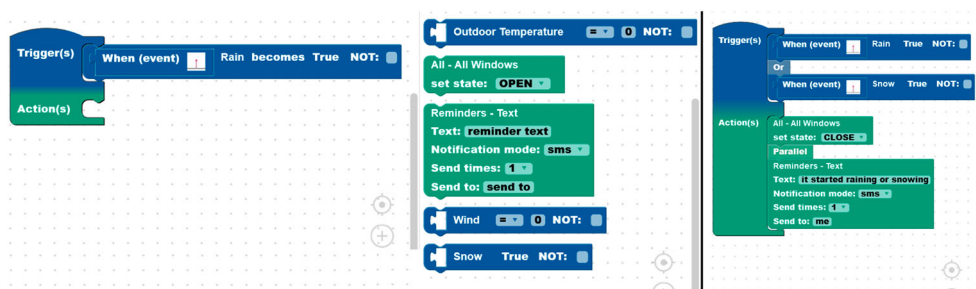
Figure 2. A comparison of the suggestions obtained when inserting ‘rain’ into the workspace: in the middle the list of step-by-step suggestions, in the right one of the ‘full rule’ recommendations.
