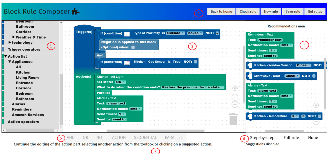
Figure 1. The main interface of the application with a rule under composition.
