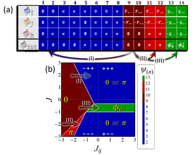
FIG. 2. (a) GSs \psi_{(n)} = (\phi_i, \phi_j, \phi_k)_{(n)} , with n = 1 \dots 14 , and a total phase value \phi_{tot} . (b) Phase diagram of the lowest-energy GS as a function of J and J_{ij} . The arrows highlight the phase transitions discussed in Fig. 3 and labeled with (I), (II), and (III). The total phase values \phi_{tot} = \{0, \pi, \text{or } \phi_0\} in the GSs are also indicated.
