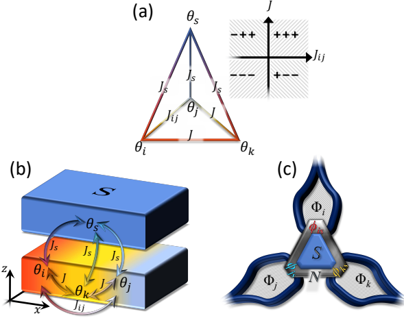
FIG. 1. (a) Schematic representation of Josephson phases assuming four phase degrees of freedom and sign-competing Josephson couplings, i.e. J_s , J_{ij} , J . (b) Sketch of the JJ made of a three-band superconductor with \pi -pairing and an s -wave single-band superconductor. The interband, J and J_{ij} , and interjunction, J_s , couplings are highlighted. (c) Equivalent circuit of the multiband JJ. The fluxes \Phi_z are used to establish the \pi -pairings.
