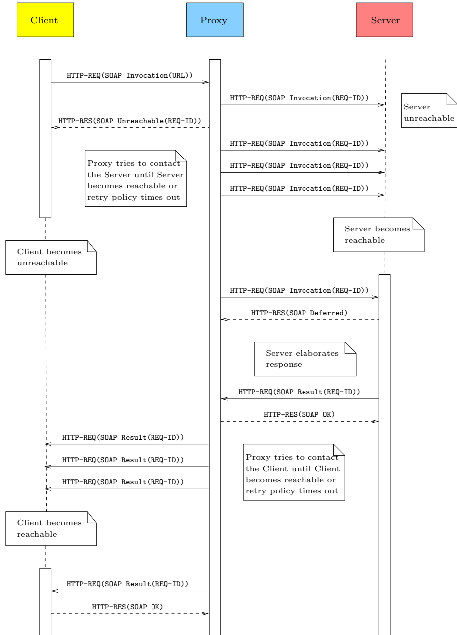
Fig. 2. Message sequence chart of an aSOAP scenario.
