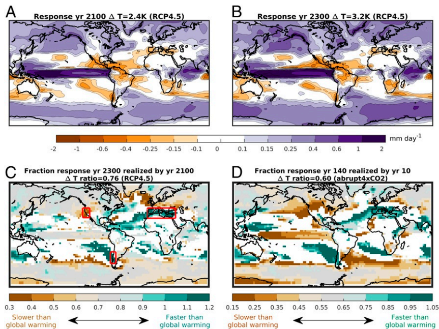
Fig. 1. (A) CMIP5 multimodel mean annual-mean precipitation response ( \text{mm-d}^{-1} ) by year 2060 to 2099 in the RCP4.5 scenario relative to 1900 to 1949. (B) As in A, but for the long-term precipitation response by year 2260 to 2299. In the titles, \Delta T indicates the global warming realized in each period. (C) Ratio of A to B, i.e., the fraction of the long-term response already realized by 2060 to 2099. Gray shading implies that the ratio in the precipitation response scales like global-mean warming. Brown (green) shading implies that the precipitation response is slower (faster) than global warming. White shading shows where less than 75% of models agree on the direction of change. (D) As in C, but for the fraction of the mean response in the abrupt4xCO 2 experiment in years 120 to 139 that is already realized by years 5 to 10. The multimodel means are based on all of the CMIP5 models available for each experiment (SI Appendix, Table S1). The results in D are confirmed both in the subset of seven CMIP5 models that form the basis of this study (SI Appendix, Fig. S1A) and in an alternative calculation where the rapid adjustment is explicitly accounted for (SI Appendix, Fig. S1B). The red boxes in C show the domains of the area-averaged values in Table 1.
