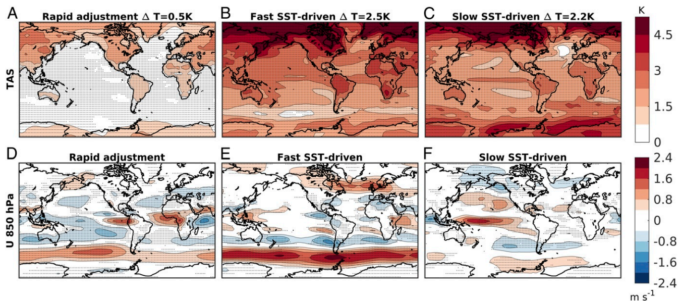
Fig. 2. (A–C) Annual-mean near-surface atmospheric temperature change (K) for the rapid adjustment (A) and for the fast (B) and slow (C) SST-driven responses to quadrupling \text{CO}_2 . The global-mean surface temperature change ( \Delta T ) is reported in the title. (D–F) As in A–C, but for the changes in the zonal wind at 850 hPa. Stippling indicates where at least 85% of the models (six out of seven) agree on the direction of change.
