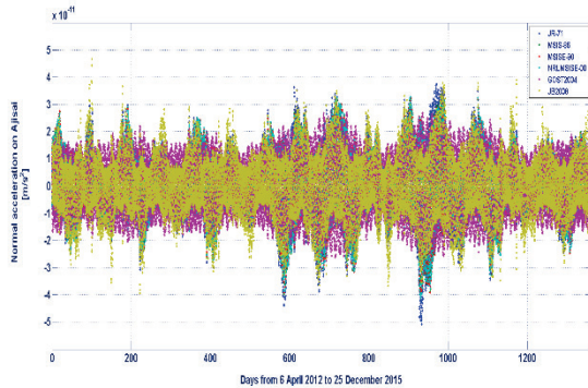
Fig. 19. Normal component ( W_D ) of the neutral drag acceleration on Ajisai, from April 6, 2012, to December 25, 2015, computed with the six atmospheric density models.
