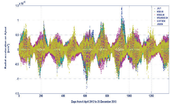
Fig. 15. Radial component ( R_D ) of the neutral drag acceleration on Ajisai, from April 6, 2012, to December 25, 2015, computed with the six atmospheric density models.
