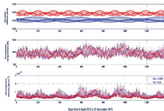
Fig. 4. Geodetic altitude of LARES and Ajisai, and corresponding exospheric temperature and atmospheric density, from April 6, 2012, to December 25, 2015, centered around the maximum of Solar Cycle 24.
