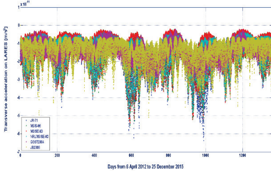
Fig. 11. Transverse component ( T_D ) of the neutral drag acceleration on LARES, from April 6, 2012, to December 25, 2015, computed with the six atmospheric density models.
