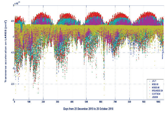
Fig. 12. Transverse component ( T_D ) of the neutral drag acceleration on LARES, from December 25, 2015, to October 26, 2018, computed with the six atmospheric density models.
