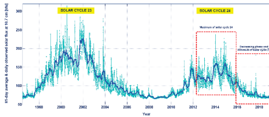
Fig. 1. Solar radio flux at 10.7 cm measured during the last two activity cycles of our star. The daily measurements and their running averages over three solar rotations (81 days) are reported.
