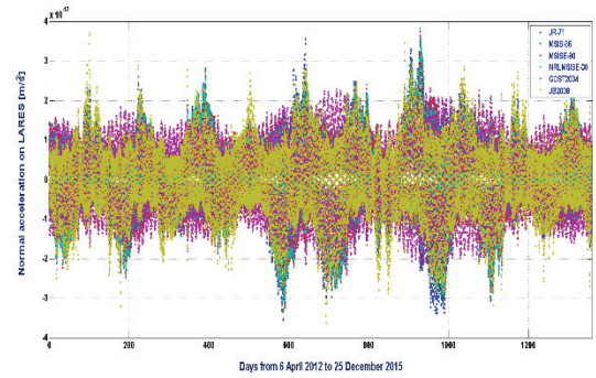
Fig. 13. Normal component ( W_D ) of the neutral drag acceleration on LARES, from April 6, 2012, to December 25, 2015, computed with the six atmospheric density models.
