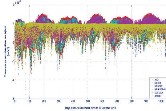
Fig. 18. Transverse component ( T_D ) of the neutral drag acceleration on Ajisai, from December 25, 2015, to October 26, 2018, computed with the six atmospheric density models.
