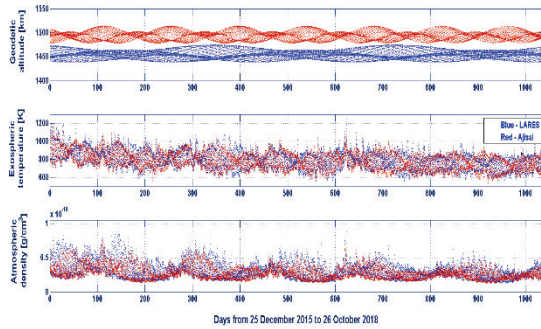
Fig. 5. Geodetic altitude of LARES and Ajisai, and corresponding exospheric temperature and atmospheric density, from December 25, 2015, to October 26, 2018, during the declining phase and the minimum of Solar Cycle 24.
