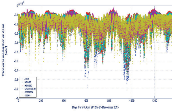
Fig. 17. Transverse component ( T_D ) of the neutral drag acceleration on Ajisai, from April 6, 2012, to December 25, 2015, computed with the six atmospheric density models.
