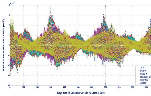
Fig. 10. Radial component ( R_D ) of the neutral drag acceleration on LARES, from December 25, 2015, to October 26, 2018, computed with the six atmospheric density models.
