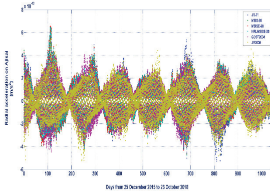
Fig. 16. Radial component ( R_D ) of the neutral drag acceleration on Ajisai, from December 25, 2015, to October 26, 2018, computed with the six atmospheric density models.
