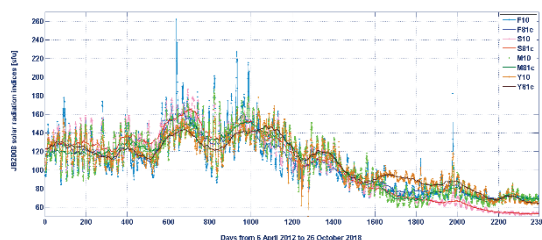
Fig. 3. Representation of the solar flux proxies used by the JB2008 thermospheric density model during the time span in which the study presented in this paper was carried out.
