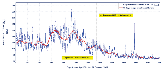
Fig. 2. Enlargement of the observed solar radio flux at 10.7 cm included in the two dashed boxes of Fig. 1. The analyses presented in this paper relate to the two time intervals separated by the vertical dashed line.
