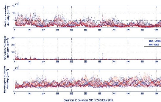
Fig. 7. Concentration of the three main atomic species, i.e. hydrogen, helium and oxygen, at the altitudes of LARES and Ajisai, from December 25, 2015, to October 26, 2018, during the declining phase and the minimum of Solar Cycle 24.
