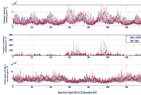
Fig. 6. Concentration of the three main atomic species, i.e. helium, hydrogen and oxygen, at the altitudes of LARES and Ajisai, from April 6, 2012, to December 25, 2015, centered around the maximum of Solar Cycle 24.
