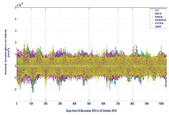
Fig. 20. Normal component ( W_D ) of the neutral drag acceleration on Ajisai, from December 25, 2015, to October 26, 2018, computed with the six atmospheric density models.
