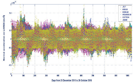
Fig. 14. Normal component ( W_D ) of the neutral drag acceleration on LARES, from December 25, 2015, to October 26, 2018, computed with the six atmospheric density models.
