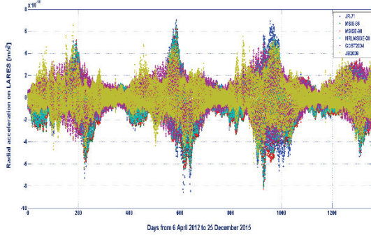
Fig. 9. Radial component ( R_D ) of the neutral drag acceleration on LARES, from April 6, 2012, to December 25, 2015, computed with the six atmospheric density models.
