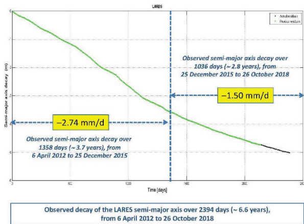
Fig. 8. Semi-major axis decay of LARES determined over 2394 days, from April 6, 2012, to October 26, 2018, processing the laser ranging data with GEODYN II.
