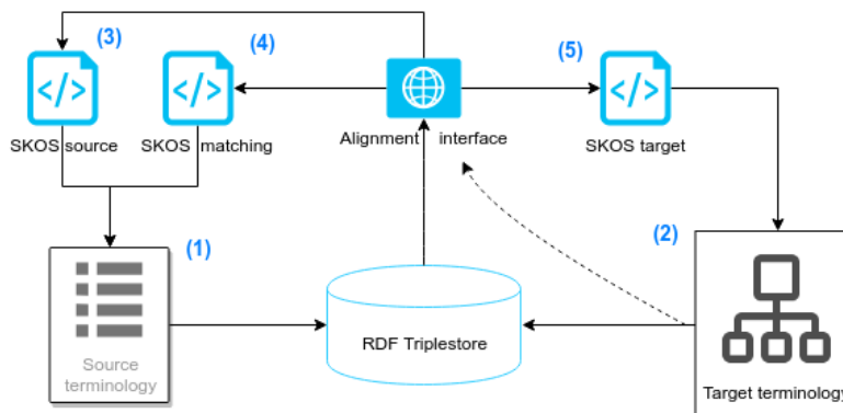
Fig. 1. Heterotoki architecture
