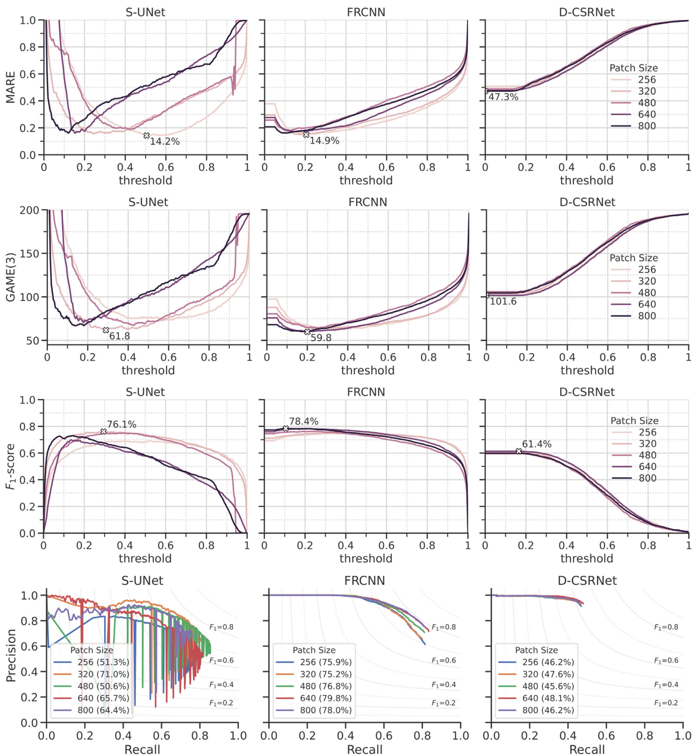
Fig. A1. PNN-MR: Impact of patch size and threshold to counting and localization performance on standard segmentation-based (S-UNet), detection-based (FRCNN), and density-based (D-CSRNet) approaches (without scoring stage). Additional results in terms of MARE, GAME(3), F1-score and Precision-Recall.
