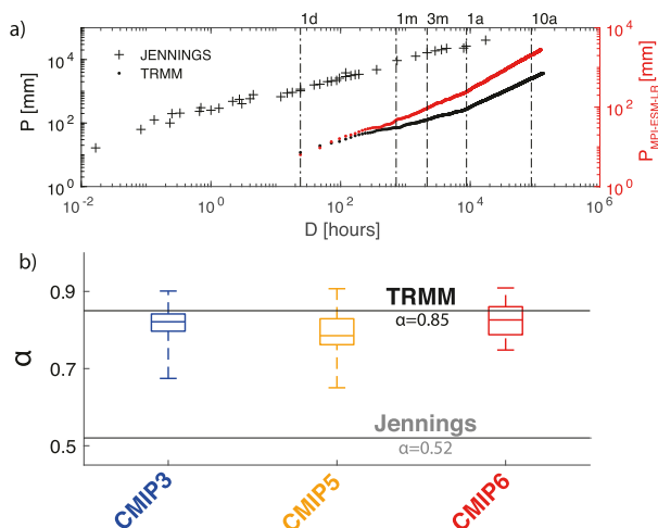
FIG. 5. Jennings scaling. (a) Three examples for the calculated data points that fall on a line in the depth-duration ( P - D ) space and (b) the Jennings slopes \alpha of that line across the CMIP phases and in TRMM, compared to the gauge measurements used by Jennings (1950). The box-and-whisker plot show the means, quartiles, and extremes across the CMIP phases.
