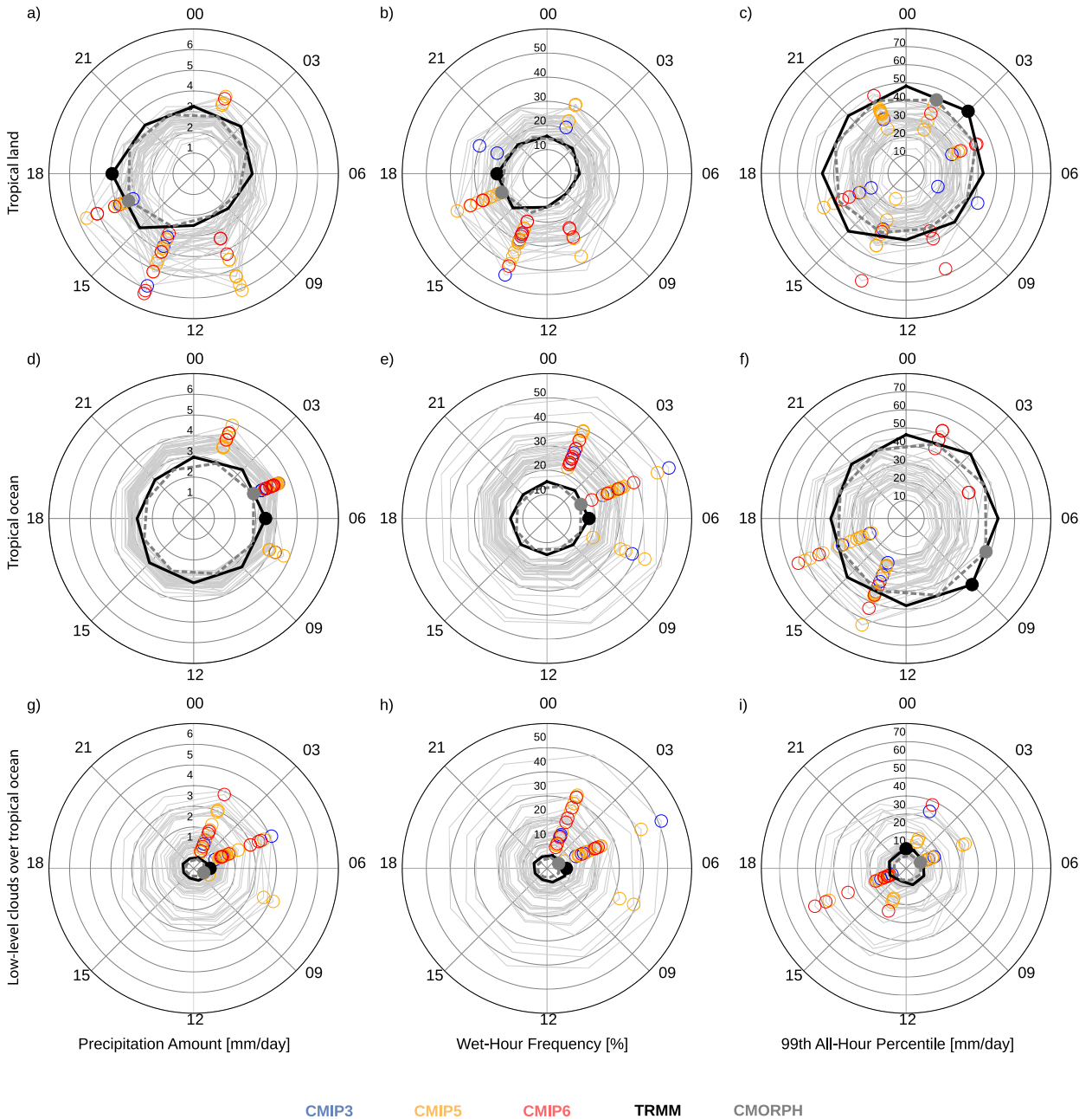
FIG. 10. Time of occurrence of tropical precipitation. The 24-h clocks show the time of the day (the angle) and the magnitude (the distance from the center) for (left) the precipitation amount, (center) the frequency of wet 3-h means, and (right) the all-hour 99th percentile of all 3-h means as index for the intensity. The analyses are shown for (a)–(c) tropical land, (d)–(f) tropical ocean, and (g)–(i) low-level clouds over tropical ocean, defined by a daily mean OLR > 250 W m -2 . The black solid (gray dashed) lines are the diurnal cycles of TRMM (CMORPH) satellite observations. Thin gray lines indicate the diurnal cycles of individual climate models to illustrate the model spread. The small circles mark the maxima in the observations and three generations of CMIP climate models. Please note that the simulations provide 3-hourly averages and are shown at the middle of the averaging period. We do not show the ensemble-averaged diurnal cycle of the CMIP phases due to the large model spread. (a)–(f) We use the 3-hourly precipitation data, marked by index 1, and (g)–(i) 3-hourly precipitation data paired with daily OLR, marked with indices 1 and 3 in Tables S1–S4.
