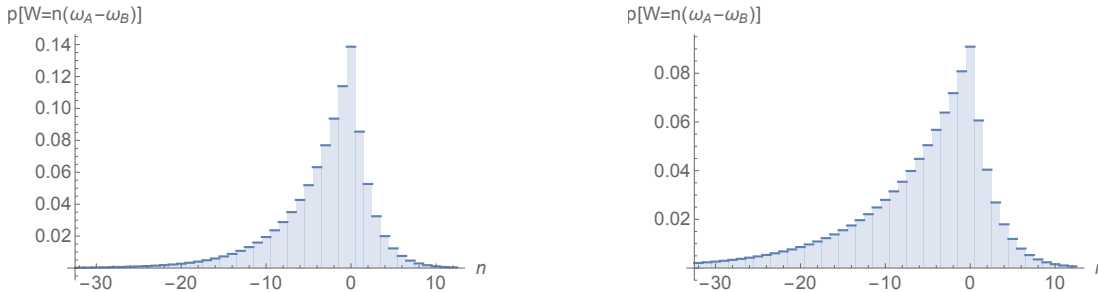
Figure 4. Distribution of the extracted work in \omega_A - \omega_B units, for N_A = 8 and N_B = 2 , for interaction strength \theta = \pi/4 (left) and \theta = \pi/2 (right). By exchanging n \rightarrow -n , the same histograms represent the probability of heat released by the hotter reservoir in \omega_A units [see Eq. (31) and (B7)].
