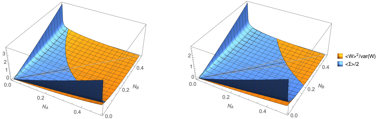
Figure 5. Plot of the signal-to-noise ratio of work \langle W \rangle^2 / \text{var}(W) and scaled entropy production \langle \Sigma \rangle / 2 for the qubit Otto engine with \theta = \pi/2 (left) and \theta = \pi/3 (right) as a function of parameters N_A and N_B .
