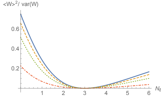
Figure 6. Signal-to-noise ratio of the work for the bosonic swap engine ( \theta = \frac{\pi}{2} ) with N_A = 3 versus occupation number N_B for ideal thermalization (solid), and finite thermalization times \gamma\tau = 3, 2 , and 1. (dashed, dotted and dot-dashed, respectively).
