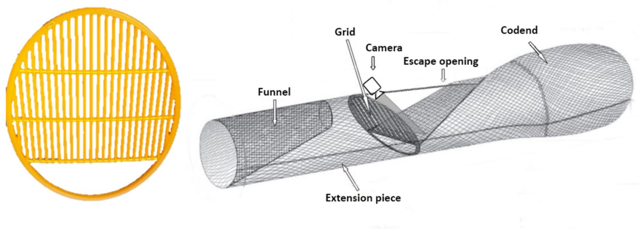
Fig. 1. Left: Juveniles' Sorting grid (JSG) selected for sea trials. Right: JSG installed in a Mediterranean trawl net, in the extension piece ahead the codend. (adapted from Bahamon et al. 17 ); the position of the camera attached to the grid is reported.
