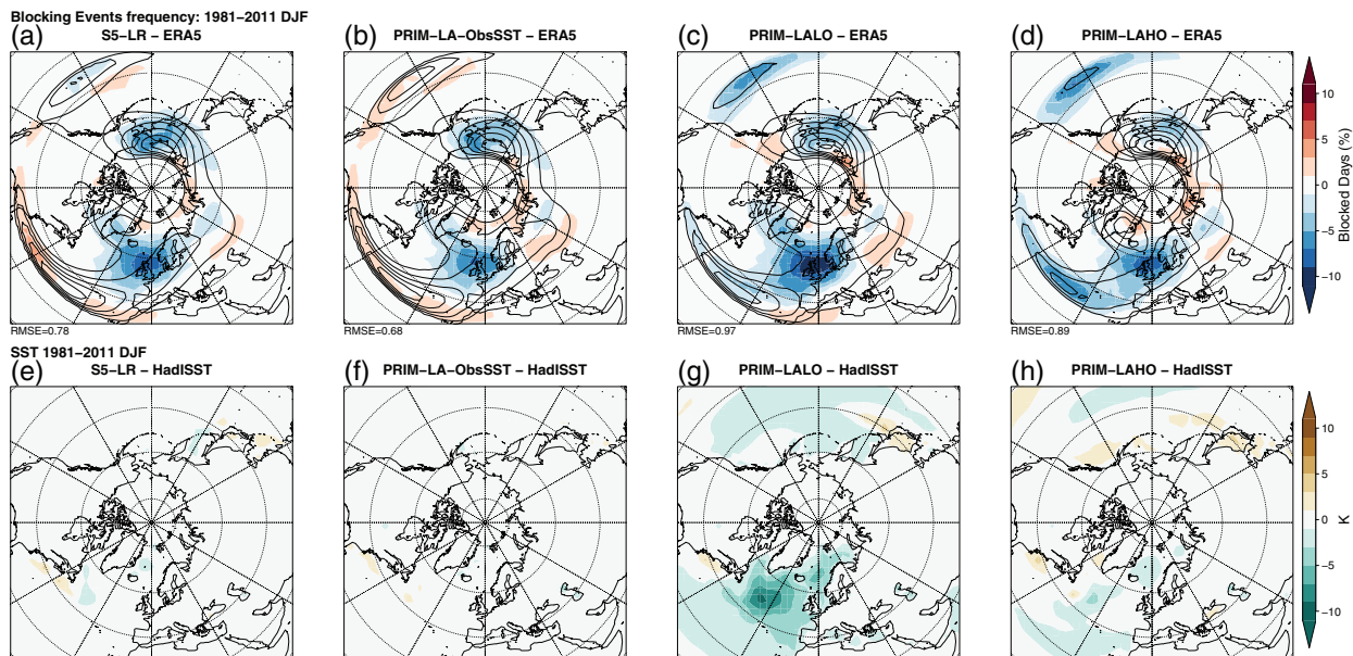
FIGURE 11 DJF 1981–2011 Blocking Events frequency for (a) S5-LR, (b) PRIM-LA-ObsSST, (c) PRIM-LALO, and (d) PRIM-LAHO (contours) and their bias against ERA5 reanalysis (shading). Contours are drawn each 3%. SST differences between (e) S5-LR, (f) PRIM-LA-ObsSST, (g) PRIM-LALO, and (h) PRIM-LAHO and the HadISST reanalysis
