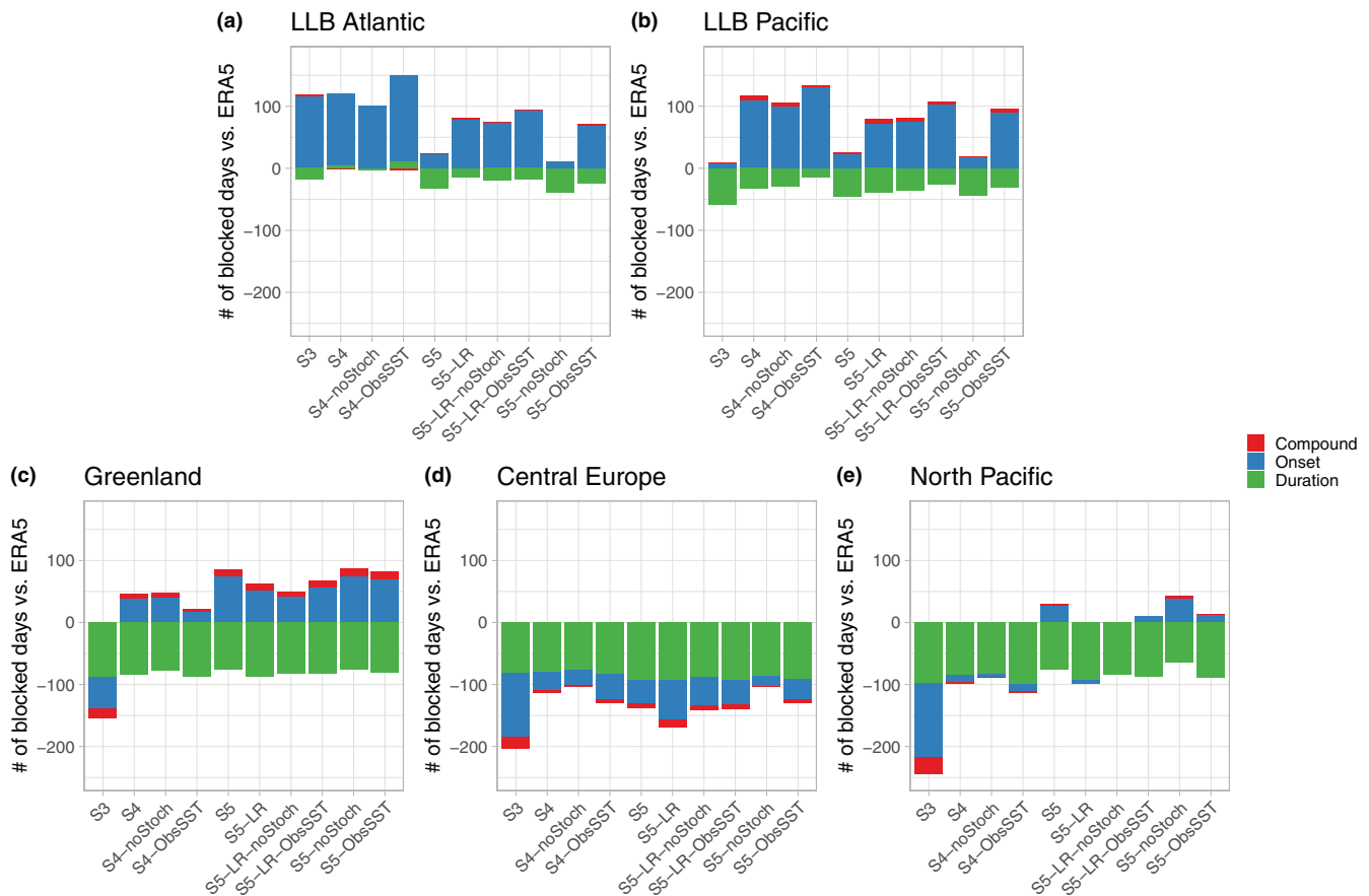
FIGURE 4 Linear decomposition of the Blocking Events frequency bias (versus ERA5) following Equation 5 into a part due to missing blocking onsets (blue), a part due to underestimated blocking duration (green), and their compound effect (red), over (a) Atlantic LLB, (b) Pacific LLB, (c) Greenland, (d) Central Europe, and (e) North Pacific sectors. Details on the linear decomposition are found in the text
