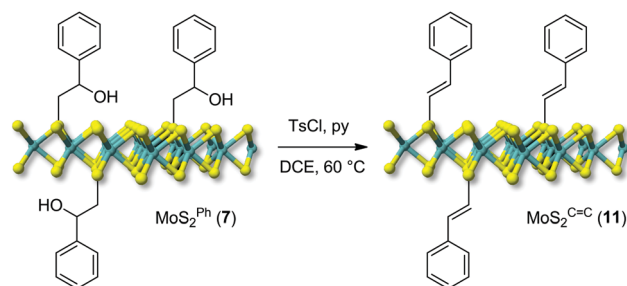
Scheme 3 Post-derivatization of the nanohybrid \text{MoS}_2^{\text{Ph}} ( 7 ) into the styrene-decorated \text{MoS}_2^{\text{C=C}} ( 11 ).
