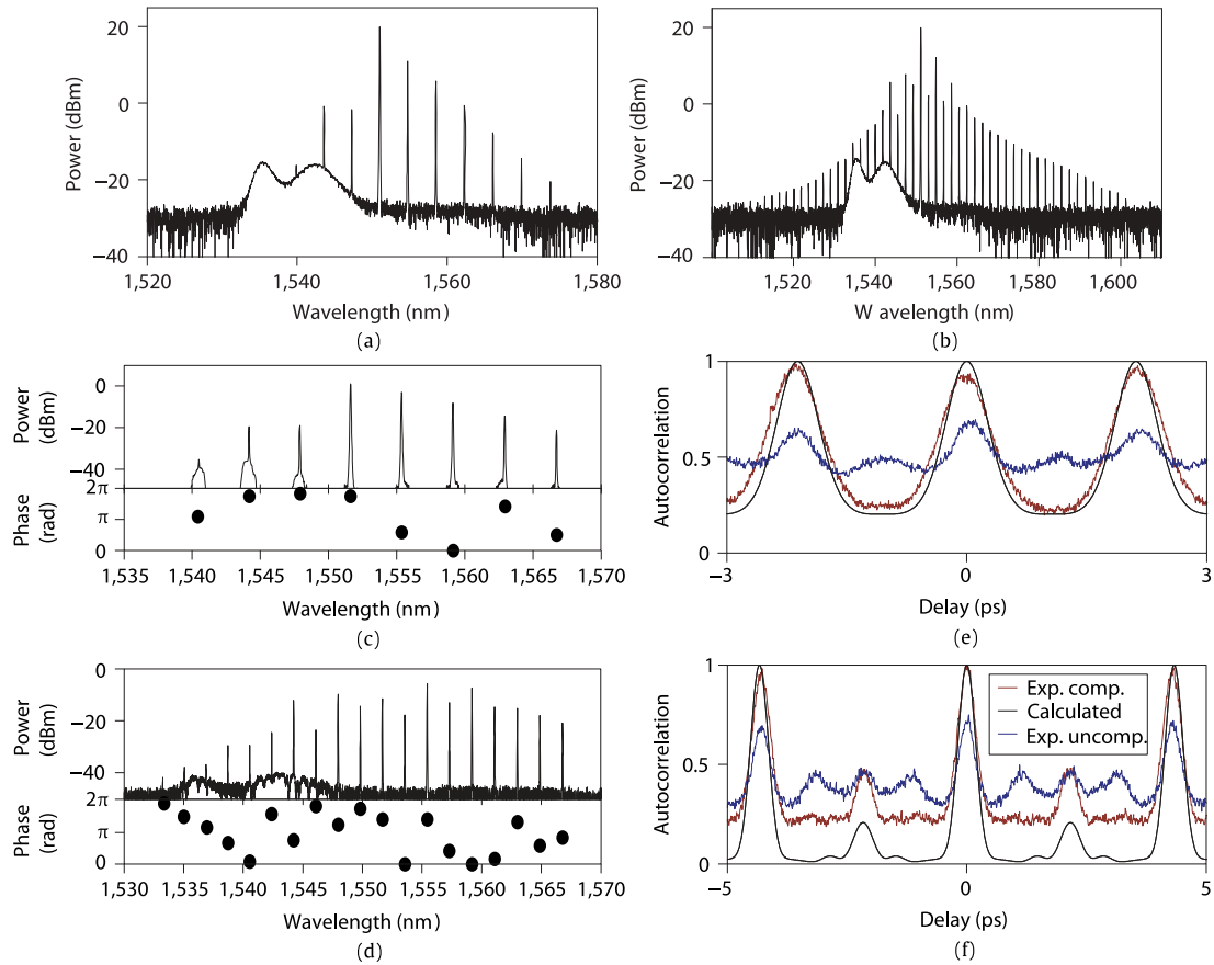
Fig. 17. Compressed pulses of Type II combs. (a), (b) Spectra after the micro-ring. The ring radius is 100\ \mu\text{m} . The pump power is 1.4\ \text{W} . The pump wavelengths are: (a) 1551.67\ \text{nm} ; (b) 1551.74\ \text{nm} ; (c), (d) Spectra after the pulse shaper (corresponding to (a), (b), respectively), together with the phase applied to each comb line for optimum SHG signals; (e), (f) Autocorrelation traces. Red lines, compressed pulse; blue lines, uncompressed pulse; black lines, calculated by taking the spectra shown in (c), (d) and assuming a flat spectral phase. (After Ref. [10].)
