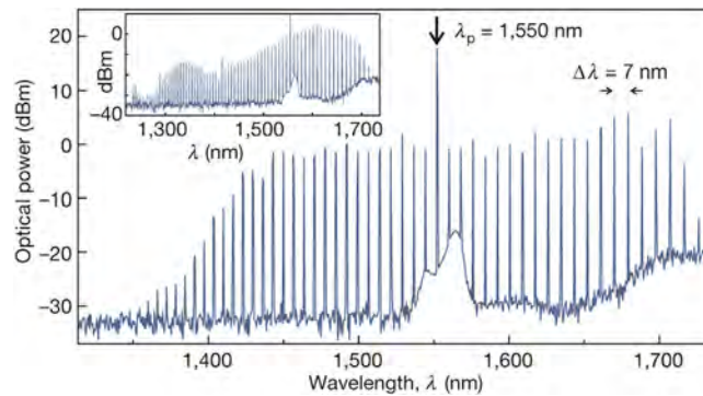
Fig. 12. Parametric frequency conversion observed in a monolithic toroid micro-cavity (pump power: 60 mW at 1550 nm). Inset: broadband emission in a different sample generating more than 70 parametric modes (pump power: 130 mW). After Ref. [8].
