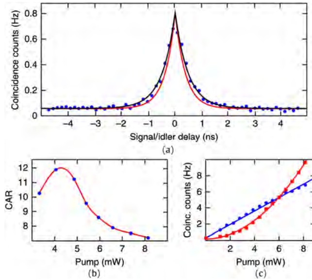
Fig. 54. Coincidence counts, coincidence-to-accidental ratio (CAR) and power scaling. (a) Measured photon coincidence peak, showing the raw measured coincidences ( C ) in Hz. The black curve corresponds to the optimum fit, resulting in a measured photon bandwidth of 320 MHz, while the red curve corresponds to the fit with the expected photon bandwidth of 410 MHz. (b) CAR as a function of balanced pump power (the line connecting the points is plotted for visual purposes), showing a CAR above 10 for balanced pump powers between 3 and 5 mW. (c) Measured photon coincidence counts (sum of all coincidence counts measured within the FWHM of the coincidence peak) for balanced and unbalanced pump powers. In the unbalanced configuration (blue circles), the TE pump power is kept constant at 6 mW and the TM pump power is increased, showing a linear-scaling behaviour. In the balanced configuration (red squares), TE and TM pump powers are identically increased, demonstrating a clear quadratic scaling behaviour without any linear contribution. After Ref. [271].
