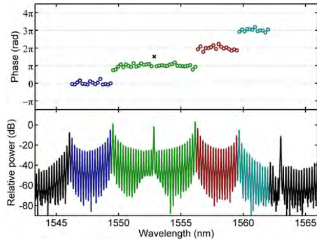
Fig. 29. Phase steps in the optical spectrum of a micro-resonator-based frequency comb. The phase of the comb modes of different sections of the micro-comb show steps of multiples of \pi .
