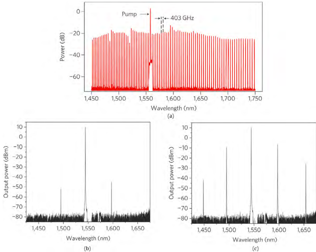
Fig. 14. Summary of the first comb observations in integrated resonators (a) OPO in a two-port silicon nitride ( \text{Si}_3\text{N}_4 ) micro-ring resonator. The measured resonator had a radius of 58 \mu\text{m} , a Q-factor of 500,000, an FSR of 403 GHz and anomalous group velocity dispersion (GVD) for \lambda < \lambda_0 = 1610 \text{ nm} . Broad spectrum operation, with lines spaced by 1 FSR, for a pump power of 310 mW at 1557.8 nm. After Ref. [11] (b–c) Four-port Hydrex micro-ring resonator (radius: 135 \mu\text{m} , FSR: 200 GHz, Q: 1.2 \times 10^6 ). Output spectra (measured at the output of the drop port) for a pump injected in the input port and tuned to a ring resonance at 1544.15 nm (pump power: (b) 50.8 mW, (c) 53.8 mW). The spectrum is generated with lines spaced by 32 FSR. After Ref. [12].
