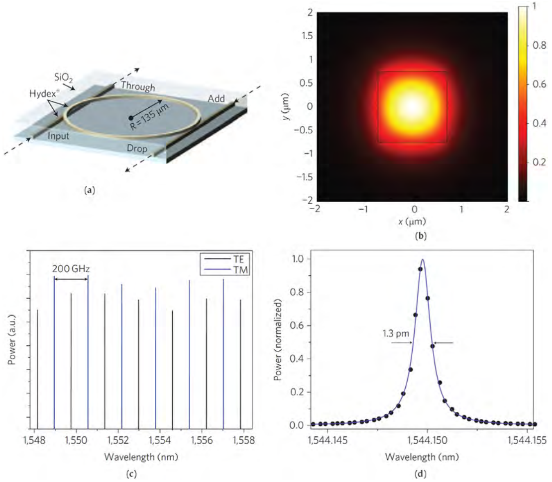
Fig. 8. Four-port Hydex micro-ring resonator (radius: 135 \mu\text{m} , FSR: 200 GHz, Q: 1.2 \times 10^6 ). (a) Drawing of the four-port device. (b) Transverse mode profile in the waveguide for the fundamental TM mode. (c) Measured resonances in the C-Band for the TE and the TM modes. (d) High-resolution measurement of a single resonance. After Ref. [12].
