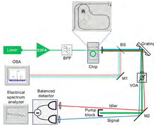
Fig. 57. Experimental set-up for squeezed state generation. The on-chip micro-ring resonator was pumped by a CW laser followed by an EDFA and a bandpass filter (BPF). To ensure efficient coupling in and out of the chip, inverse tapers, together with a lensed fibre, were used. The output of the waveguide was collected with a high-NA objective lens. The diffraction grating spatially separated the pump and the twin beams. After blocking the pump, the beams were focused onto a balanced detector. The RF output of the balanced detector was sent to an RF spectrum analyser. A small fraction of the beams was sent to an OSA to monitor the onset of parametric oscillation. The inset shows a microscope image of the ring-resonator coupled to the bus waveguide. The shape of the fabricated ring is noncircular to fit the resonator within one field of the electron-beam lithography tool, thus avoiding stitching errors. VOA: Variable optical attenuator. M1, M2: Mirrors. BS: Beam splitter. After Ref. [333].
