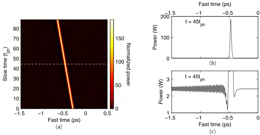
Fig. 26. Time-domain characteristics of a CS perturbed by higher-order dispersion. (a) Temporal evolution showing how the CS exhibits a time-domain drift. (b) Temporal CS profile at t = 45t_{\text{ph}} , indicated by the dashed line in (a). A zoom on the leading tail of the CS is shown in (c).
