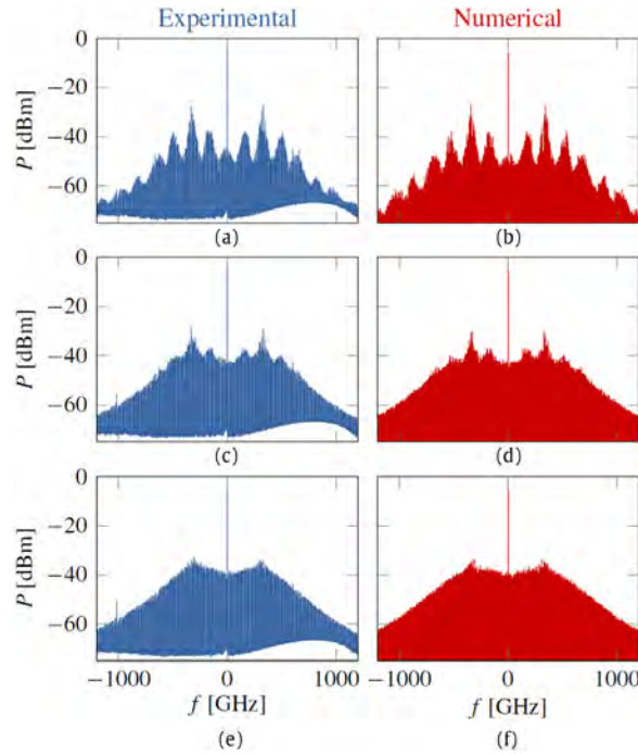
Fig. 31. Experimental observation of chaotic comb states in an 11-mm-diameter MgF 2 resonator with a mode spacing of 6 GHz. Panels (a), (c), (e) show measurements of chaotic micro-comb spectra, with the corresponding simulated comb states in panels (b), (d), (f). \Delta is 0.3, 1.8 and 2.7 for (b), (d), (f), respectively. Different values for \Delta correspond to different de-tunings between the pump laser frequency and the micro-resonator resonance frequency. After Ref. [242].
