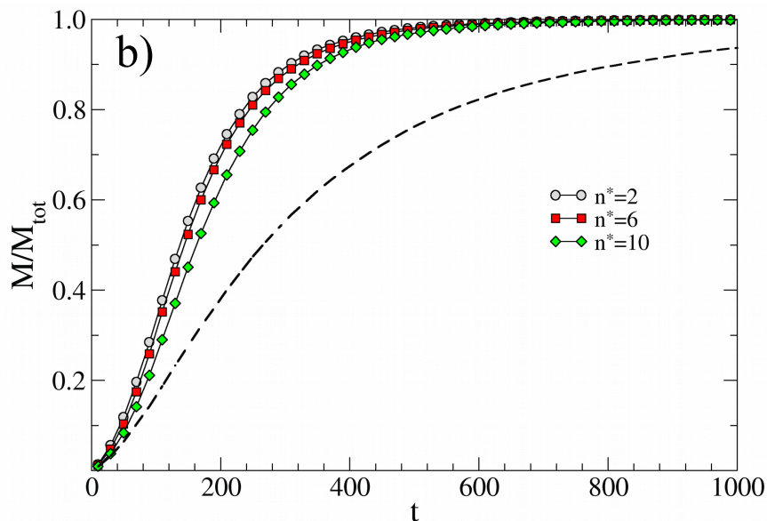
FIG. 1. a) Schematic of the protein aggregation model describing the main processes involved: primary nucleation occurring with rate k_M (and correspondingly k_n in mean-field), polymer elongation with rate k_H ( k_+ in mean-field), secondary nucleation with rate k_S ( k_2 in mean-field) and diffusion with rate k_D which is not described by mean-field theory. b) Simulations showing the dependence on the minimal polymer size n^* needed to catalyze secondary nucleation of the aggregation curve, the polymer mass fraction M/M_{\text{tot}} , obtained for k_M = 4 \cdot 10^{-4} , k_D = 10^{-2} , k_S = 1 , k_H = 10^4 and \rho = 0.16 . The dashed line is the curve obtained in the limit n^* \rightarrow \infty , or equivalently in absence of secondary nucleation.
