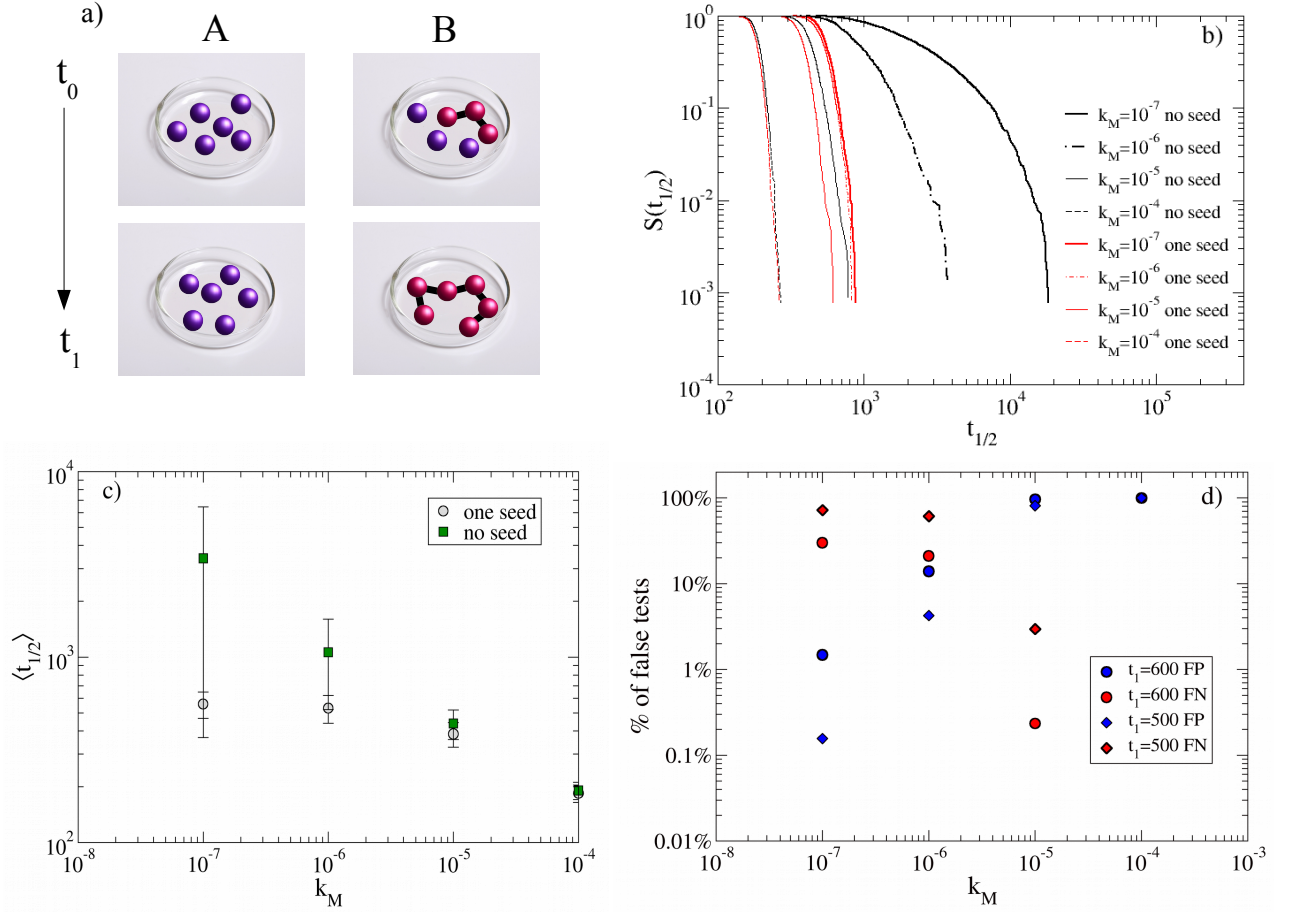
FIG. 10. Intrinsic fluctuations rule errors in the detection of protein aggregation prone samples. a) A test to detect seeds for protein aggregation is based on small volume sampling of protein solutions at time t_0 = 0 and on the assumption that only seeded samples (e. g. sample B) would form aggregate at time t_1 . b) Simulations allow to compute the distribution of half-times for samples with and without a seed as a function of the rate of primary nucleation k_M . Data are obtained sampling over n = 1200 independent realization. c) Average half-time ( \pm standard deviation) as a function of the rate of primary nucleation k_M . d) Fraction of false positives (FP) and false negatives (FN) for testing times t_1 = 600 and t_1 = 500 . Time is measured in units of 1/k_S , N = 1250 .
