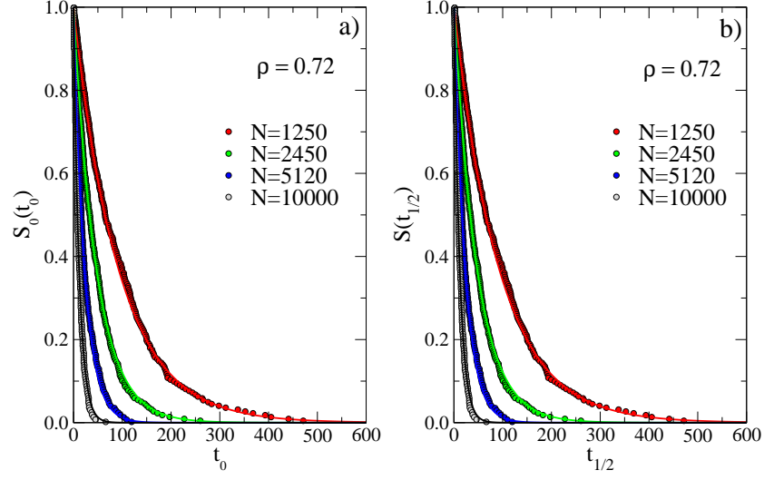
FIG. 6. The complementary cumulative distribution functions S(t_0) (a) and S(t_{1/2}) (b) for four different monomer numbers N and density \rho = 0.72 . The symbols correspond to the numerical simulations while the lines represent the theoretical predictions obtained from Eq.(6) and Eq.(7). Here k_D = 10^{-2} and k_M = 4 \cdot 10^{-6} .
