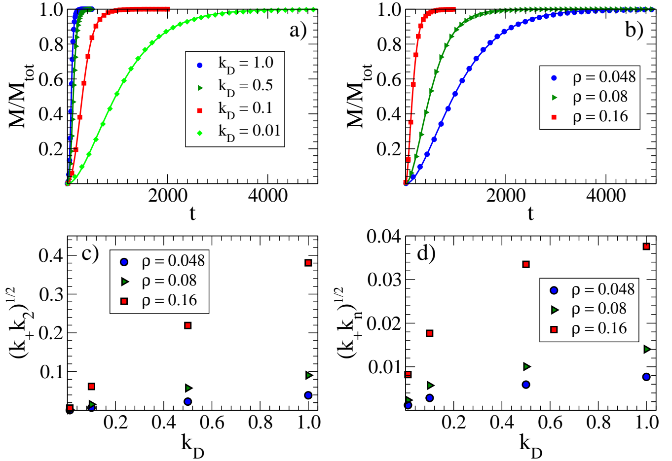
FIG. 2. Protein aggregation depends on monomer diffusion: a) Simulations showing the diffusion dependence of the aggregation curve, the polymer mass fraction M/M_{\text{tot}} , obtained for k_M = 4 \cdot 10^{-4} , k_S = k_H = 1 , N = 2450 and \rho = 0.048 . The curves are well fit by mean-field theory (full lines) with effective parameters that depend on k_D . b) Simulations of the density dependence of the polymer mass fraction for N = 2450 , k_M = 4 \cdot 10^{-4} , k_H = 1 and k_D = 10^{-2} . Fits by mean-field theory are plotted as lines with effective parameters reported in the panels c) and d). Time is measured in units of 1/k_S . c)-d): The effective mean-field parameters \sqrt{k_+ k_2} and \sqrt{k_+ k_n} obtained by fitting simulations performed for k_M = 4 \cdot 10^{-4} , k_S = k_H = 1 as a function of the concentration \rho and the diffusion rate k_D .
