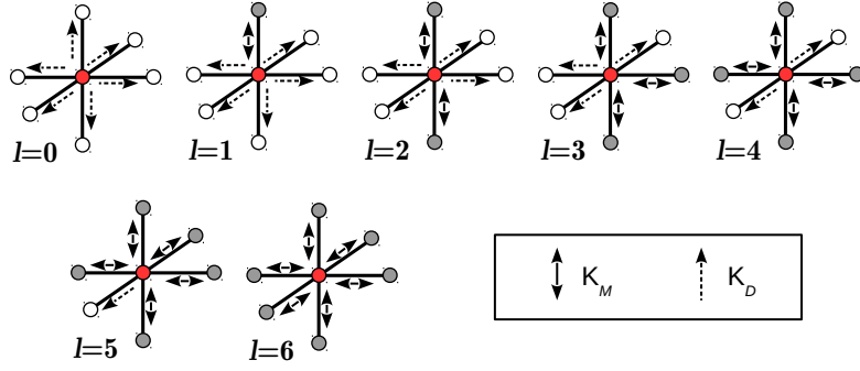
FIG. 8. A schematic representation of the possibilities of diffusion (dashed arrow) and aggregation (double arrow) for a monomer (red circle) placed in the center of cubic lattice unit cell. The monomer partners for the dimerization (from l = 1 to l = 6 ) are colored in grey while the empty sites are represented by white circles. The aggregation and diffusion rate are, respectively, k_M and k_D .
