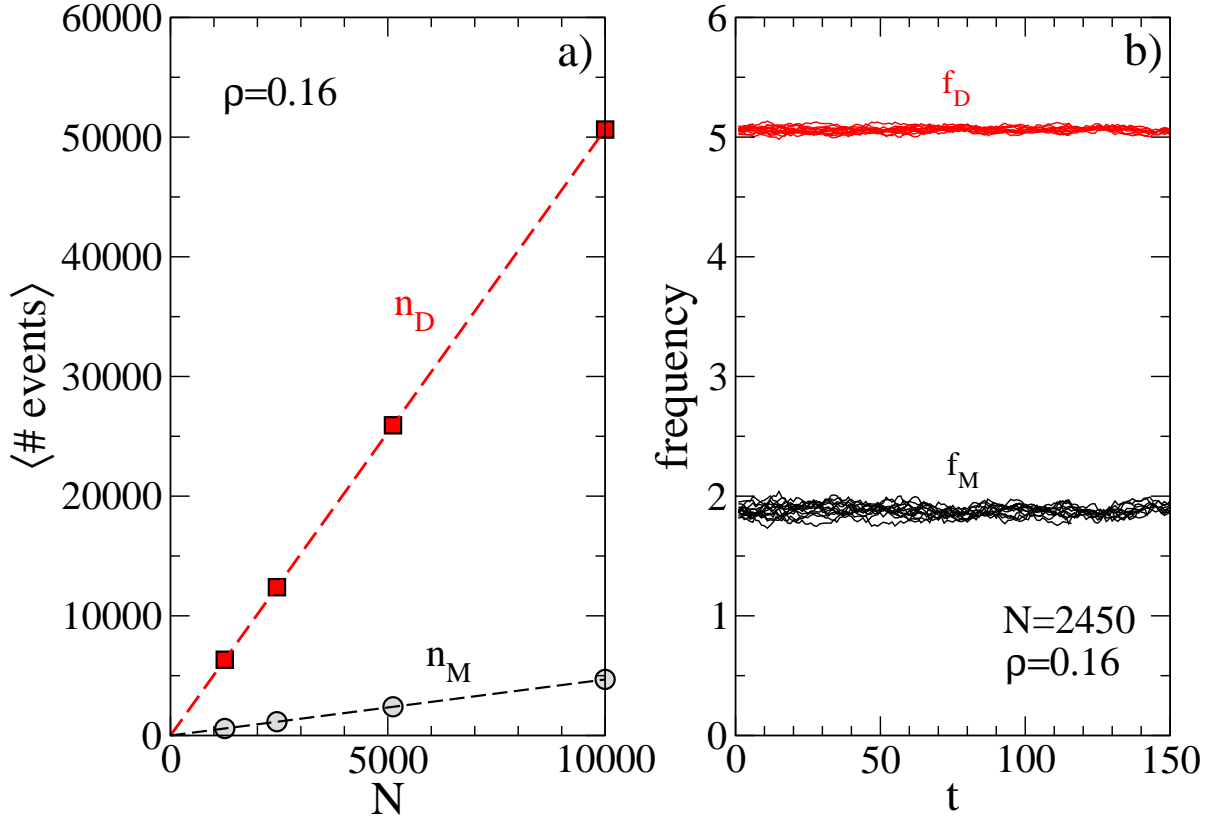
FIG. 9. a) The number of possible primary nucleation and diffusion events ( n_M and n_D , respectively) are a linear function of the number of monomers N . b) The corresponding frequencies f_M and f_D fluctuate very little in time. Here k_D = 10^{-2} , k_M = 4 \cdot 10^{-6} , N = 2450 and \rho = 0.16 .
