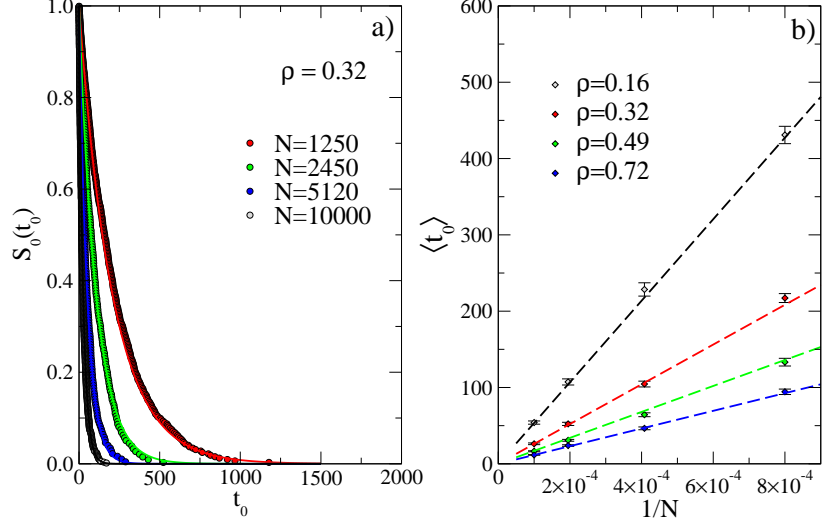
FIG. 4. a) The complementary cumulative distribution functions S(t_0) for four different monomer numbers N and density \rho = 0.32 . The symbols correspond to the numerical simulations while lines correspond to the theoretical predictions obtained from Eq. (6). b) The average time \langle t_0 \rangle as a function of 1/N for four different number densities. The theoretical predictions (dashed lines) are obtained from Eq.(13). Here k_D = 10^{-2} and k_M = 4 \cdot 10^{-6}
