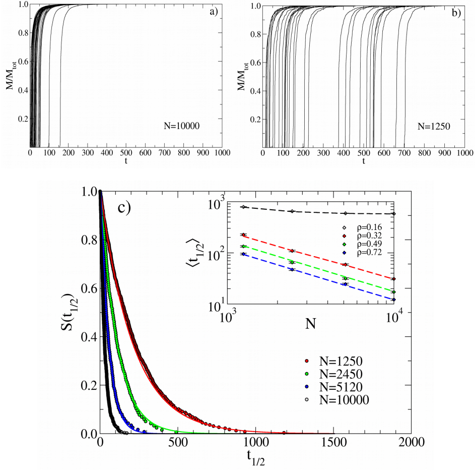
FIG. 3. Half-time sample-to-sample fluctuations are due to extreme value statistics. Different replicates of the simulations display wide fluctuations in half-times especially for small numbers of monomers. a) Simulation results obtained for N = 10000 monomers at \rho = 0.32 , k_M = 4 \cdot 10^{-6} , k_S = 1 , k_H = 10^4 , k_D = 10^{-2} . The graph shows that the half-time t_{1/2} is very close to the nucleation time t_0 at which the curves depart from zero. b) Same as panel a) but with N = 1250 . c) The complementary cumulative distributions of half-times obtained from simulations for different values of N are in agreement with the theory described in the text. The inset shows that the average half-times for different concentrations \rho as a function of N . The general trend is in agreement with experiments [13]. Time is measured in units of 1/k_S .
