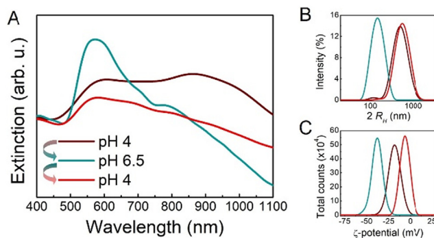
Fig. 5. Modulation of the Lyz-AuNPs assembling and optical properties by acting on the pH of the solution: representative extinction spectra (A), hydrodynamic diameter (B) and \zeta -potential (C) distributions of 100 nm Lyz-AuNPs prepared at x = 2000 .
