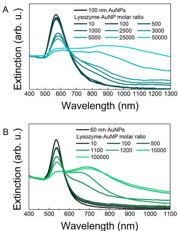
Fig. 4. Representative extinction spectra acquired at different Lyz-AuNP molar ratios for 100 nm (A) and 60 nm (B) AuNPs. The spectra measured for the corresponding AuNPs stock solutions are also shown for comparison.
