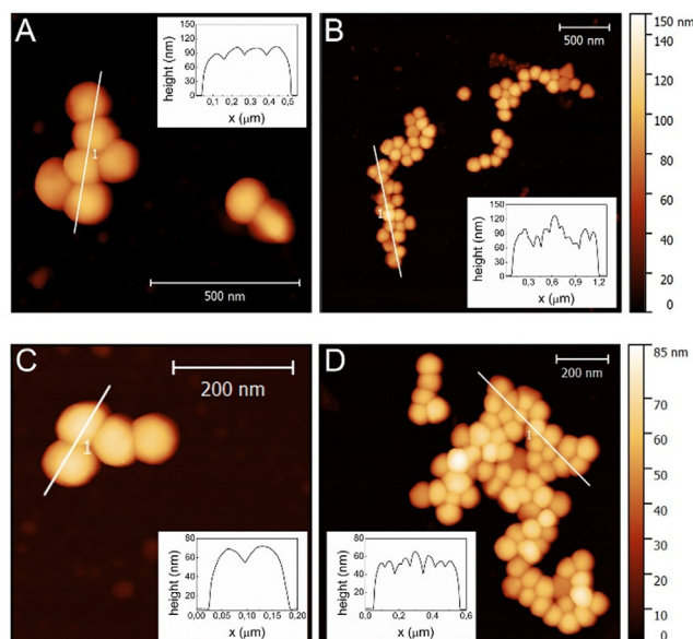
Fig. 3. Representative AFM images acquired on clusters corresponding to x = 3000 (A) and x = 10000 (B) for 100 nm AuNPs and to x = 1200 (C) and x = 5000 (D) for 60 nm AuNP. The corresponding height profiles are reported in the insets.
