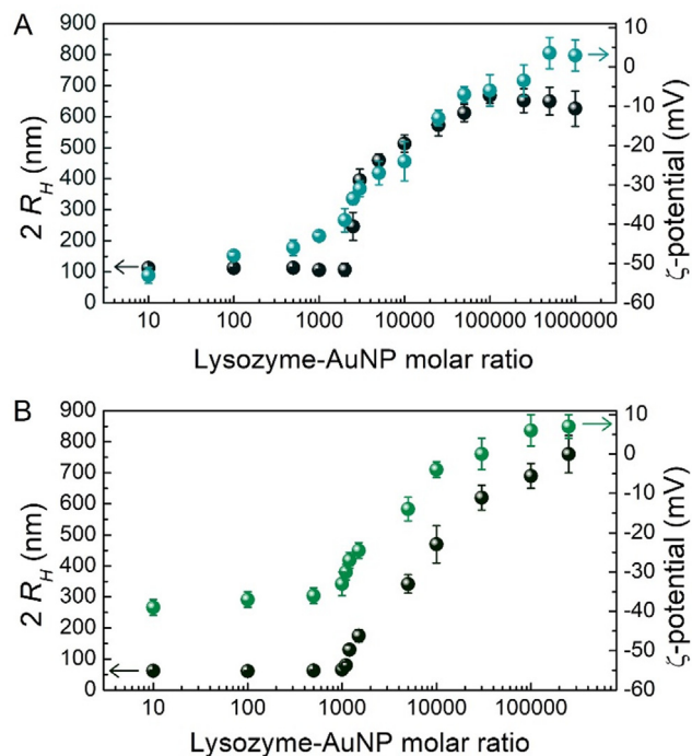
Fig. 2. DLS measurements (hydrodynamic diameter, 2R_H , and \zeta -potential trends) on Lyz-AuNPs as a function of the lysozyme-AuNPs molar ratio, using AuNPs of 100 nm (A) and 60 nm (B). Each reported value is obtained by three measurements.
