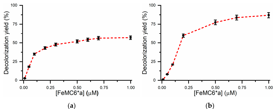
Figure 4. Decolorization percentage of NR (110 \mu M (a)) and MB (9.9 \mu M (b)) as a function of the FeMC6*a concentration. The reaction was performed in 100 mM phosphate buffer, pH 6.5, 3 mM H_2O_2 . The dashed line between each point was intended as a guide for the eye, while the error bars defined a 10% confidence level.
