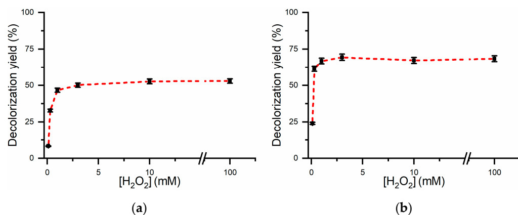
Figure 5. Decolorization percentage of NR (110 \mu M (a)) and MB (9.9 \mu M (b)) as a function of the H_2O_2 concentration. The reaction was performed in 100 mM phosphate buffer, pH 6.5, 0.5 \mu M FeMC6*a. The dashed line between each point was intended as a guide for the eye, while the error bars defined a 10% confidence level.
