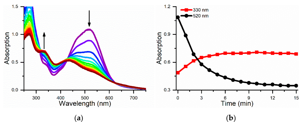
Figure 7. NR (0.12 mM) degradation followed by UV–Vis absorption spectroscopy. Spectra were acquired every minute for 15 min (colored lines from violet to red) (a). The absorption band decrease at 520 nm is accompanied by the formation of a band at 330 nm (b). The reaction was performed in 100 mM phosphate buffer, pH 6.5, 1.0 \mu\text{M} FeMC6*a, and 0.10 mM \text{H}_2\text{O}_2 .
