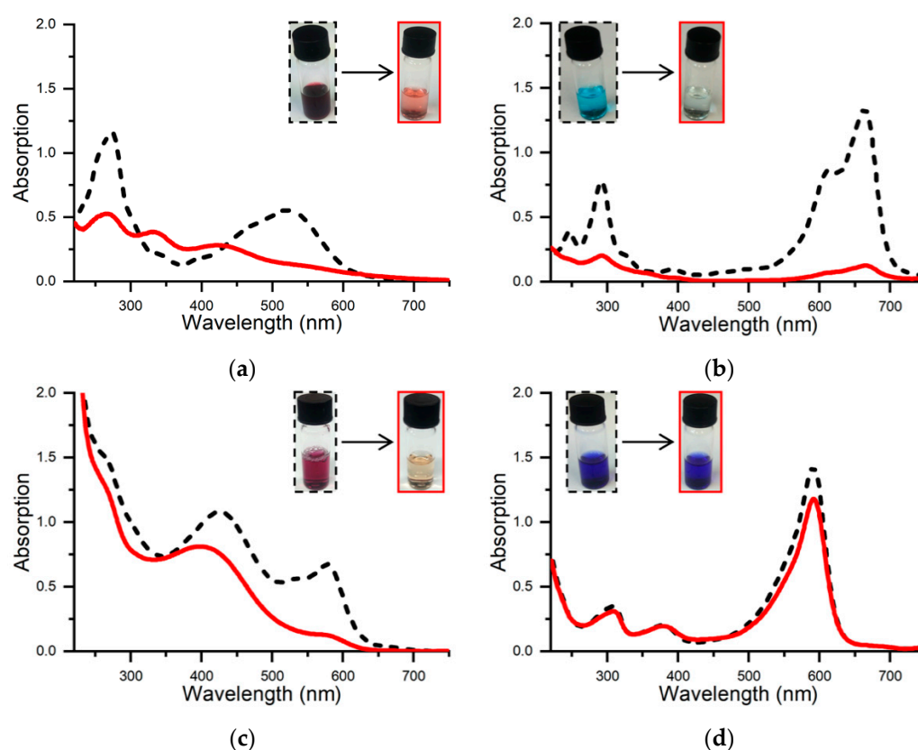
Figure 3. Decolorization process as followed by UV–Vis spectroscopy. Two spectra are reported for each dye, the first before the addition of H 2 O 2 (black dashed line) and the second after the addition of H 2 O 2 , when no further consumption of the dye was observed (red line). All the reactions were performed in a solution of the dye and 1 \mu M FeMC6*a in 100 mM phosphate buffer, pH 6.5, to which 0.25 mM H 2 O 2 was added. Dye oxidation was monitored over 15 min for NR (60 \mu M, (a)), MB (12.9 \mu M, (b)), XO (78 \mu M, (c)), and BPB (13.5 \mu M, (d)). Insets show the photographic pictures of the reaction mixtures before (left) and after (right) decolorization.
