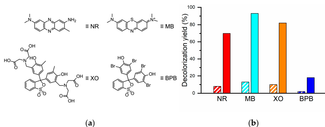
Figure 2. Structures of the dyes tested in this work. (a) Neutral Red (NR), Methylene Blue (MB), Xylenol Orange (XO), and Bromophenol Blue (BPB) are shown in one representative resonance/tautomeric structure over several possible ones. The bar plot (b) reports the decolorization percentage for NR (110 \mu M, red), MB (12.9 \mu M, cyan), XO (78 \mu M, orange), and BPB (13.5 \mu M, blue) when 1 \mu M FeMC6*a was absent (left, half filled) or present (right, filled) in the reaction mixture (100 mM phosphate buffer, pH 6.5, 0.25 mM H 2 O 2 ).
