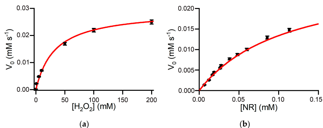
Figure 8. Oxidation activity of FeMC6*a. (a) Initial rate dependence towards the \text{H}_2\text{O}_2 concentration. The reaction conditions were FeMC6*a (1 \mu\text{M} ) and NR (25 mM) in 100 mM phosphate buffer, pH 6.5. (b) Initial rate dependence towards NR concentration. The reaction conditions were FeMC6*a (1 \mu\text{M} ) and \text{H}_2\text{O}_2 (0.10 M) in 100 mM phosphate buffer, pH 6.5. The data points were fitted using the Michaelis–Menten equation (red lines), and the error bars corresponded to the standard deviation of three repetitions.
