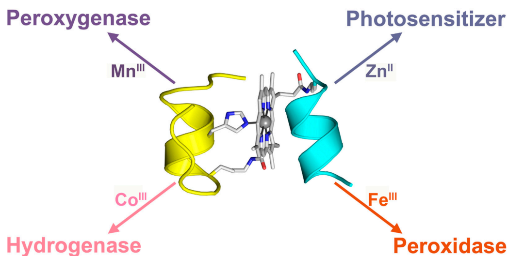
Figure 1. MC6*a designed model and its dominant enzymatic activities exhibited with different metals.
