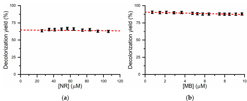
Figure 6. Decolorization percentage of NR (a) and MB (b) as a function of their respective concentrations (26–106 \mu\text{M} and 0.72–10 \mu\text{M} , respectively). The reaction was performed in 100 mM phosphate buffer, pH 6.5, 0.5 \mu\text{M} FeMC6*a, and 3.0 mM \text{H}_2\text{O}_2 . The dashed line between each point was intended as a guide for the eye, while the error bars defined a 10% confidence level.
