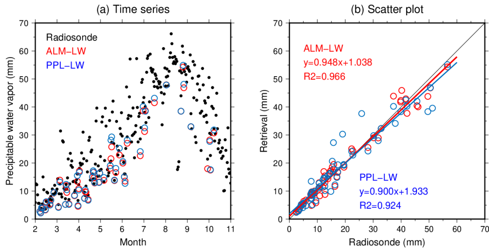
Figure 12. Seasonal changes (a) and scatter plots (b) for the precipitable water vapor of the ALM-LW (red), PPL-LW (blue), and radiosonde observations (black); y = ax + b and R^2 are the linear fitting and coefficient of determination.
