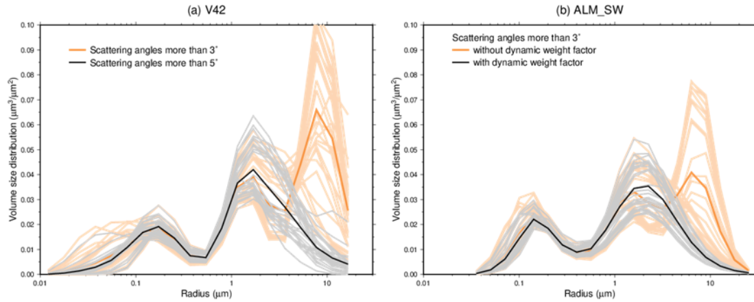
Figure 8. Retrieved volume size distribution in Tsukuba on 14 March 2018. (a) The results of the Skyrad v4.2 using the diffuse radiances at scattering angles more than 3° (orange) and 5° (gray and black). (b) The results of MRI v2 using the diffuse radiances at a scattering angle more than 3° and with (gray and black) and without (orange) the dynamic weight factor in Eq. (5). The thick lines are daily means.
