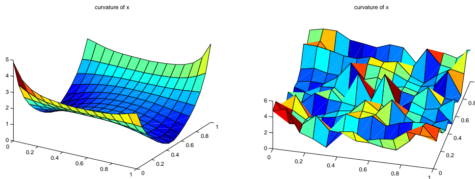
Figure 17: Solution of MPS computed by AL-RMTR-MF (left) and BOSS-SQP (right).
