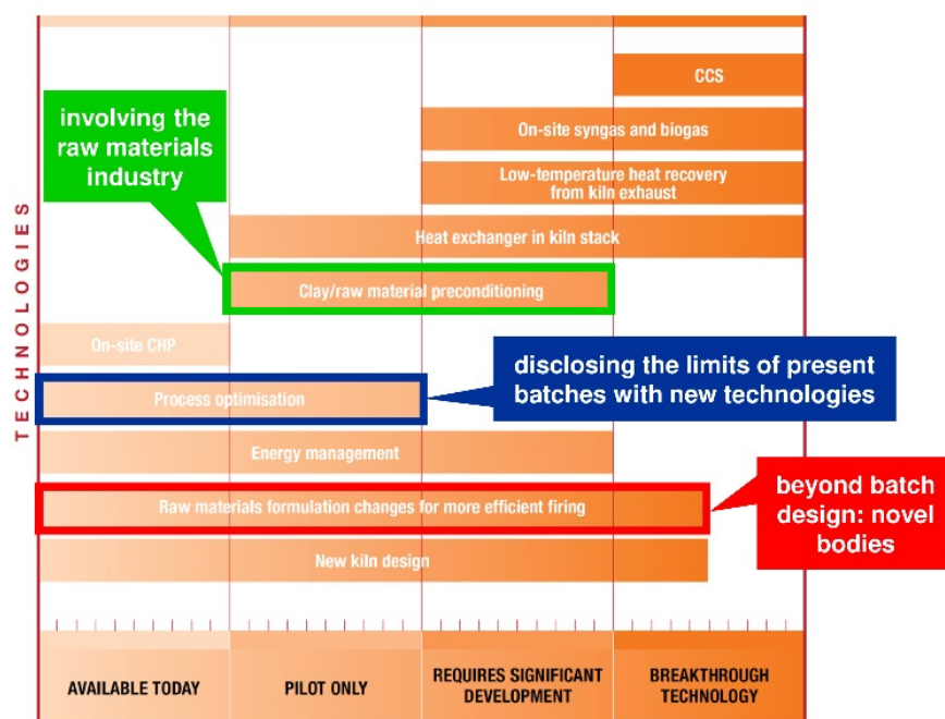
Figure 2. Key-enabling technologies concerning raw materials claimed in the Roadmap for the ceramic industry to 2050 [30].
