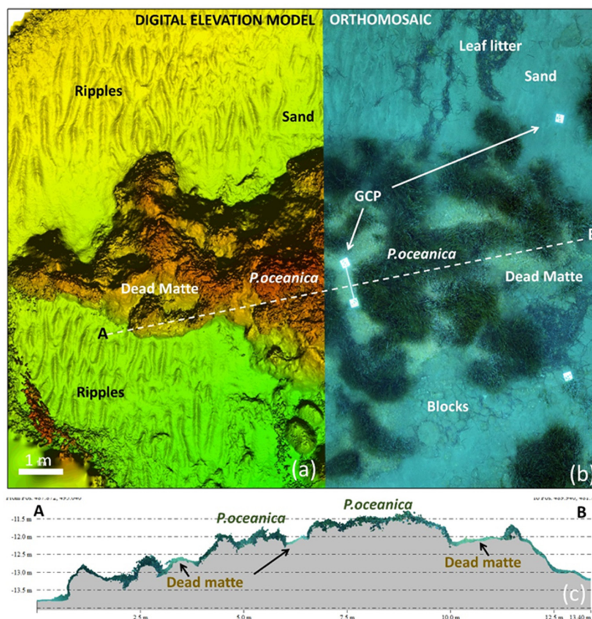
Figure 15. (a) Digital Elevation Model of P. oceanica meadows on matte at Ventotene Island. (b) Orthomosaic and DEM integration of P. oceanica . (c) AB bathymetric profile of leaf canopy height.
