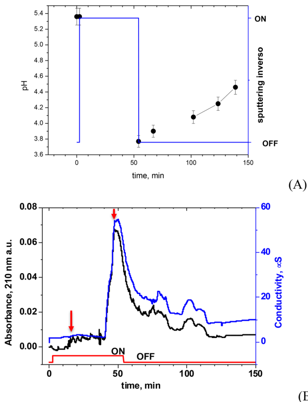
FIG. 4. (a) Trend of pH during the experiment after switching on/off the PLO generator (water flow = 1 l/h, O_2 pressure = 1 bar, 10 min inverse sputtering electron device time, and ddp = 15.000 V). (b) Online measurements of conductivity and absorbance at 210 nm of PLO solution sampled.
