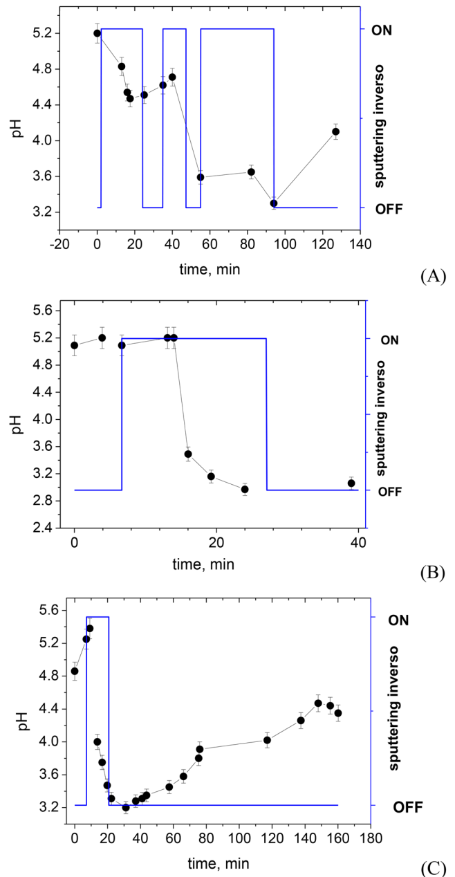
FIG. 3. Three representative experiments (A), (B), (C) in which the pH of the PLO solution sampled in B was measured (N = 3 replicates for each sampling).
