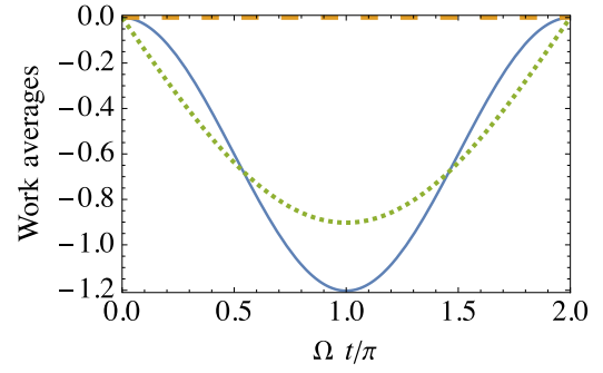
FIG. 4. Average work in units of \Omega for the spin-1/2 model described in Sec. IV C as a function of the final protocol time t_2 = t . We consider the parameters p = 1/2 , c = -1/2 , and \Omega = (1 + \sqrt{2})\delta . In particular, we plot the average \langle W \rangle of the KDQ distribution of work (blue solid line), the average work \langle W \rangle_{\text{TPM}} returned by the TPM scheme (orange dashed line)—equal to zero for any time—and the classical bound from Eq. (135) (green dotted line) taken with opposite sign.
