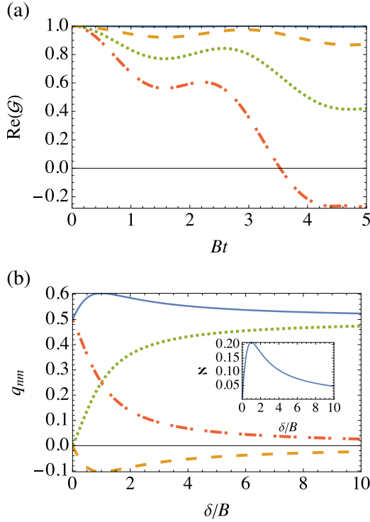
FIG. 8. (a) Real part of LE \mathcal{G}(t) as a function of time for different values of \delta : 0.1 (blue solid line), 0.4 (orange dashed line), 0.7 (green dotted line), 1.0 (red dot-dashed line). (b) Quasiprobabilities q_{nm} associated with the LE of Eq. (187) as a function of \delta/B : q_{00} (blue solid line), q_{01} (orange dashed line), q_{10} (green dotted line), q_{11} (red dot-dashed line). Inset: nonpositivity functional \aleph [see Eq. (25)] as a function of \delta/B .
