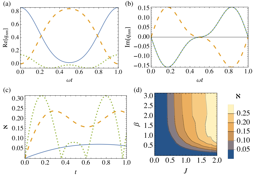
FIG. 7. We plot the real and imaginary parts of q_{nm} in panels (a),(b) respectively, as a function of \omega t , for J = 2 (lines, blue solid: nm = 11 , orange dashed: nm = 10 , green dotted: nm = 00 ). The nonpositivity functional \aleph [see Eq. (25)] is shown in panel (c), as a function of time for different values of the coupling J (lines, blue solid: J = 0.5 , orange dashed: J = 1.5 , green dotted: J = 2.5 ). (d) Contour plot of the the minimum value of \aleph in the time interval 0 \leq t \leq 20 as a function of \beta and J . Other parameters: u = \pi/2, B_1 = 1, B_2 = 1.1, \beta = 10 .
