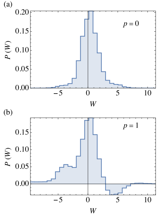
FIG. 9. KDQ distribution of work for the Ising model undergoing a sudden change of the Hamiltonian \mathcal{H}(\lambda) . Specifically, the Ising spin chain with N = 12 spins is quenched from \lambda_0 = 0 to \lambda_1 = 0.5 . Panel (a), p = 0 . Panel (b), p = 1 . Other parameters: \beta = 0.1 .
