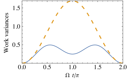
FIG. 5. Plot of the work variances of the KDQ (real part, blue solid line) and TPM (orange dashed line) distributions, respectively. The parameters are the same as in Fig. 4.
