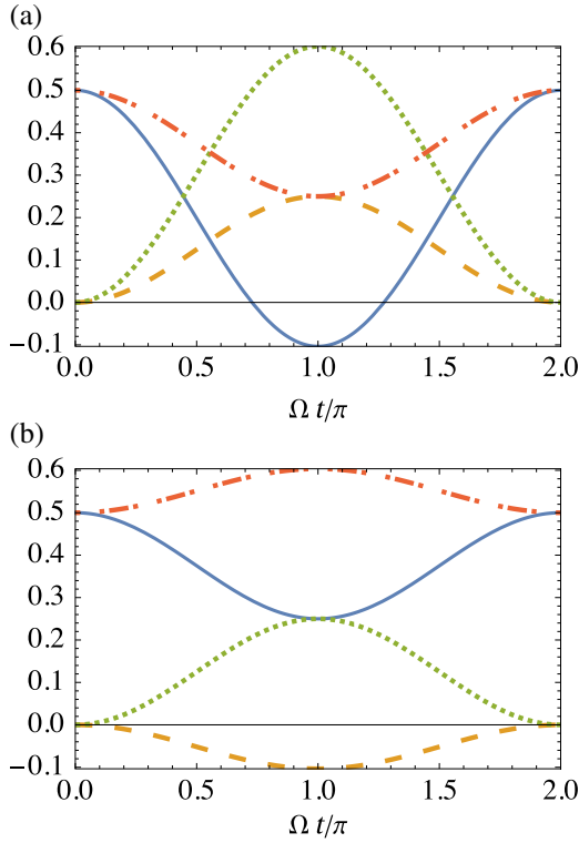
FIG. 3. Real parts of the quasiprobabilities q_{ij} defined in Eqs. (120)–(123) (with p = c = 1/2 ) as a function of time t = t_2 for \Omega = (\sqrt{2} - 1)\delta in panel (a) and \Omega = (\sqrt{2} + 1)\delta in panel (b). \text{Re}[q_{--}] (blue solid line), \text{Re}[q_{+-}] (orange dashed line), \text{Re}[q_{-+}] (green dotted line), \text{Re}[q_{++}] (red dot-dashed line).
