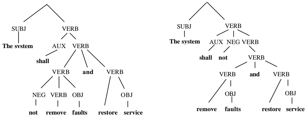
Figure 3: Two possible derivation trees
