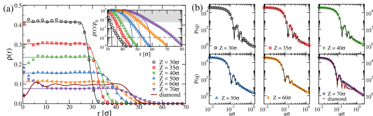
Figure 4. (a) Monomer density profiles for c = 3.2\% microgels at different confinement radius Z as a function of the distance r from the microgel center of mass. Here symbols are simulation results; lines are obtained from the fits of the form factors using the fuzzy sphere model and applying eq 8. The inset shows the same data rescaled by the polymer density of the inner core, which changes with Z , on a log–linear scale. The shaded area shows the approximate extent of the region where the curves obtained through eq 8 well-reproduce the numerical data. The value of r at which each data set intersects the dashed gray line defined by \rho(r)/\rho_0 \equiv 10^{-3} provides an estimate of the hydrodynamic radius, R_H . (b) Form factors P(q) for microgels generated with different confinements. Symbols are simulation data, and lines are fits to eq 6. The (dark red) thick lines in (a) and in the bottom-rightmost panel of (b) refer to a microgel generated by a diamond-lattice configuration.
