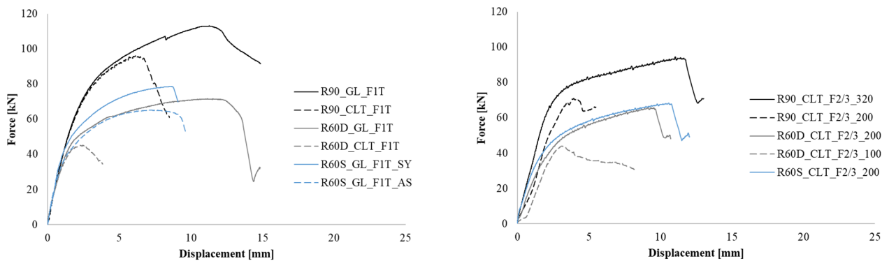
Figure 7. Force-displacement backbones: FIT (left) and F2/3 (right)
