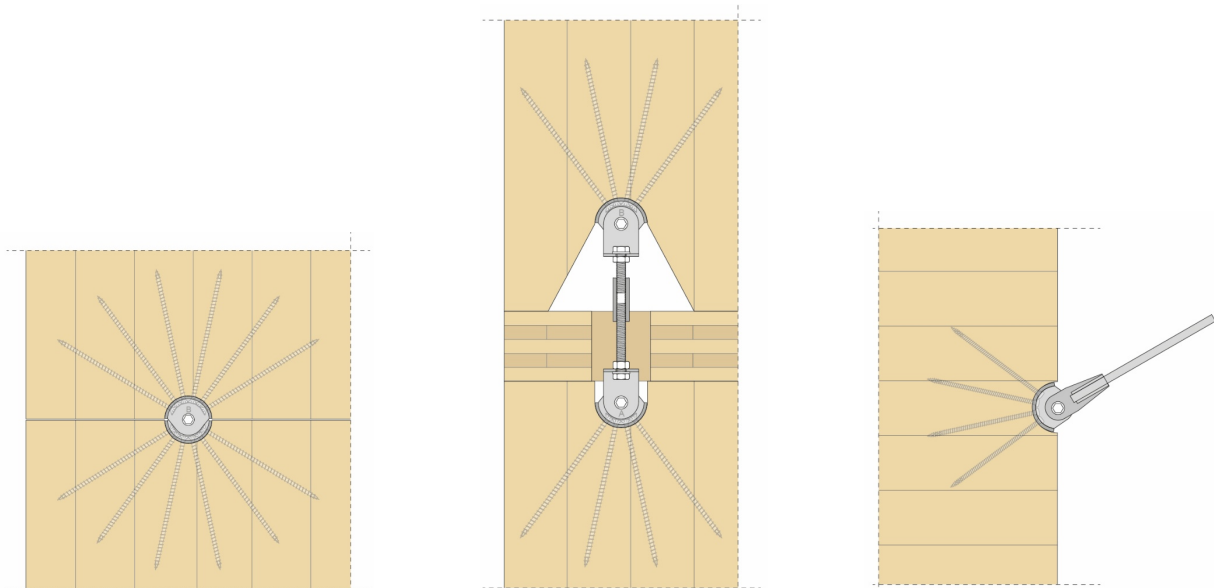
Figure 2. RADIAL connectors: direct coupling (left), coupling with RADIALKIT (centre) and anchoring system for bracing elements (right)
