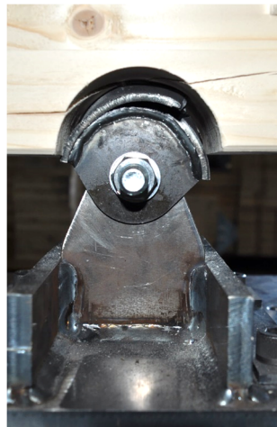
Figure 5. FIT failure modes RADIAL90: steel plate (left) and screws withdrawal failure mode (right)
