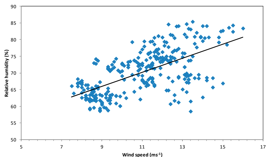
Figure 11. Variation of the relative humidity versus wind speed for an onshore wind direction (marine air mass episode). The data were recorded on the island of Porquerolles by Piazzola (personal communication). The black line fits the data.
